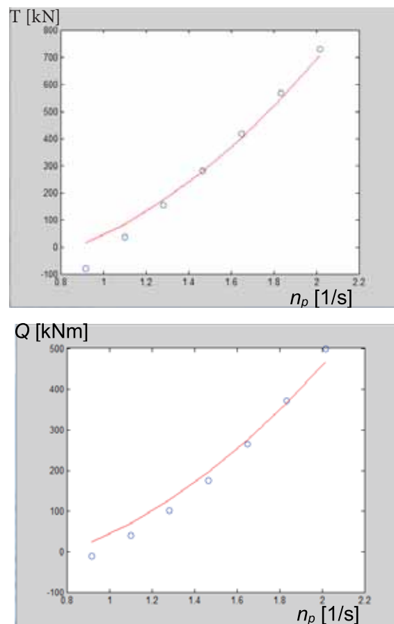
Fig. 2. Propeller thrust and torque values calculated by means of the developed approximations (4) (points marked „o”) as well as by using the hydrodynamic characteristics of the screw propellers installed on the existing bulk carriers
