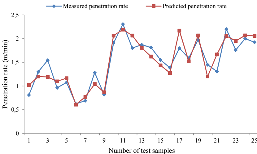
Fig. 4. Comparison between the measured and the predicted penetration rate for ANN model
