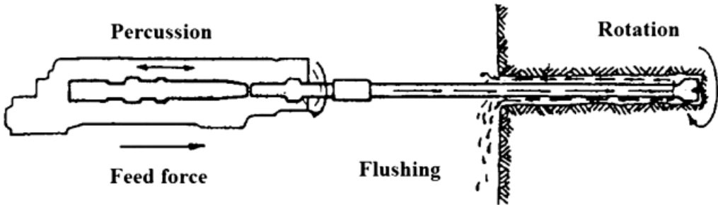
Fig. 1. A typical Top Hammer drill (Jimeno, 1995)
