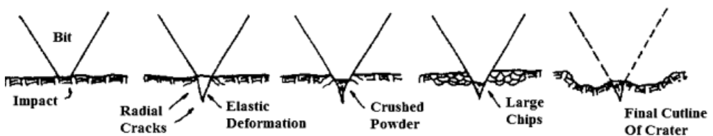
Fig. 2. Sequence of rock failure during center formation (Hartman, 1959)
