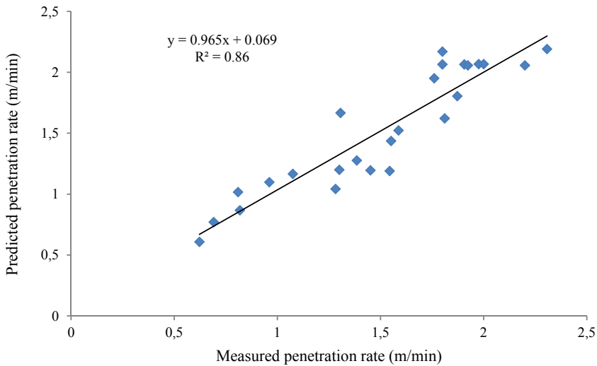
Fig. 5. Correlation between measured and predicted penetration rate for ANN model
