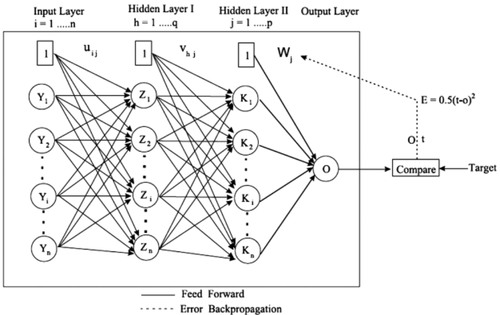
Fig. 3. A typical neural network with two hidden layers (BPNN) (Neaupane & Achet, 2004)
