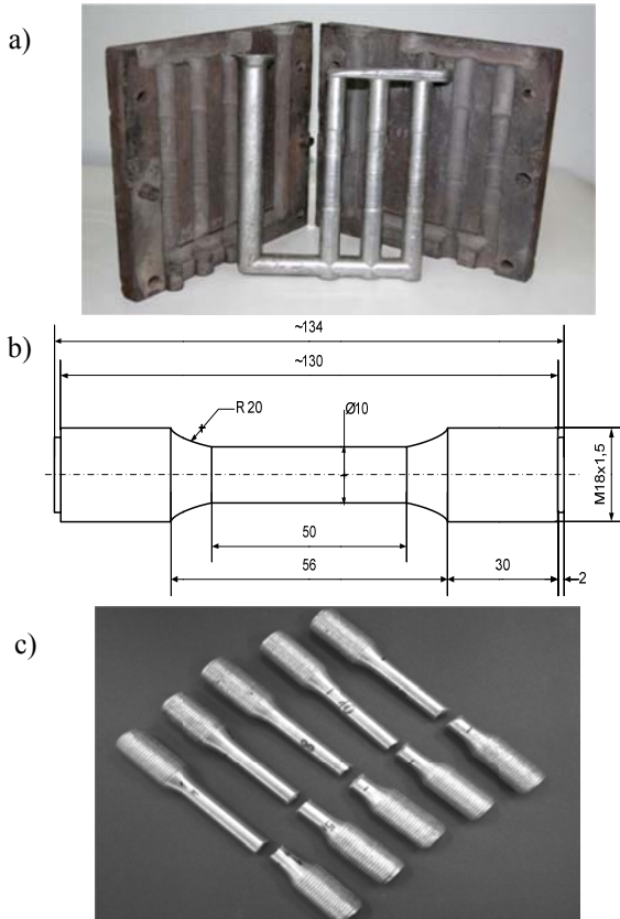
Fig. 1. Metal mould along with the casts (a), die diagram of static tensile test (b) and samples after rupture (c)
