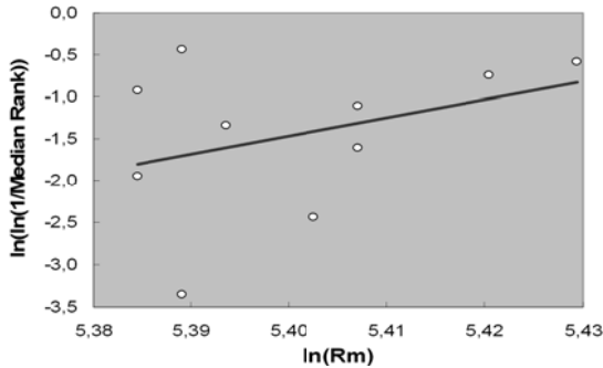
Fig. 2. The correlation diagram of population A of the AISi alloy
