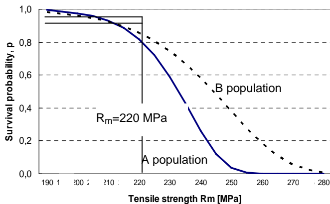
Fig. 4. Survival diagram for A and B population of AlSi alloy
