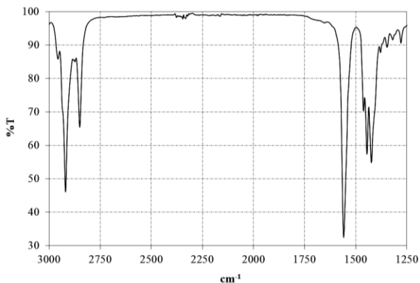
Fig. 9. Reference FTIR spectrum of NaOI
