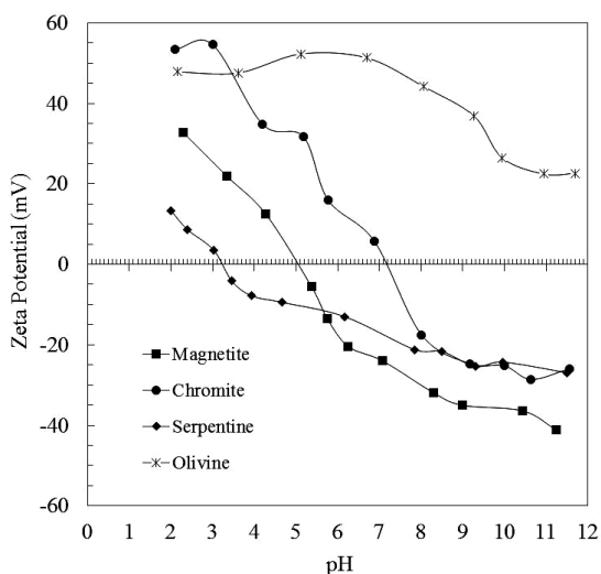
Fig. 2. Zeta potential of magnetite, chromite, serpentine (Ucbas et al., 2014) and olivine
