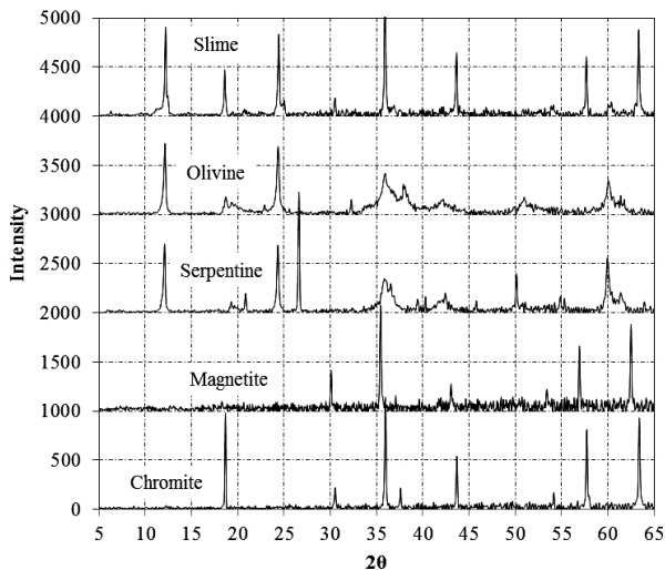
Fig. 1. XRD analysis of investigated minerals (Ucbas et al., 2014), olivine and chromite slime
