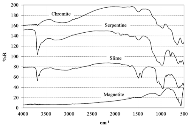
Fig. 8. Reference DRIFT spectra of minerals (Ucbas et al., 2014) and the slime sample
