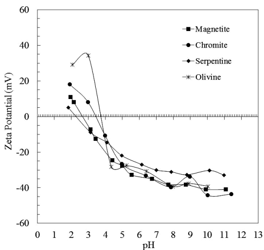
Fig. 3. Zeta potential of minerals in 2 \cdot 10^{-5} M NaOl solution
