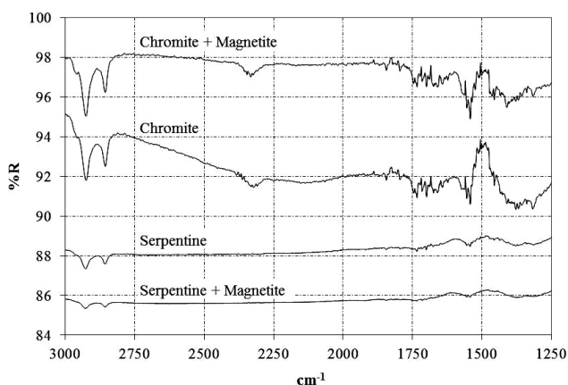
Fig. 11. DRIFT spectra of chromite and serpentine in the presence of magnetite
