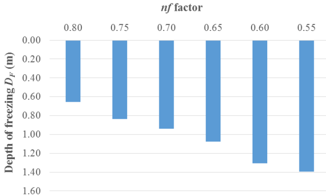
Fig. 5. Achieved values of the freezing depths D_F of track substructure in the railway track model for various boundary climatic conditions
