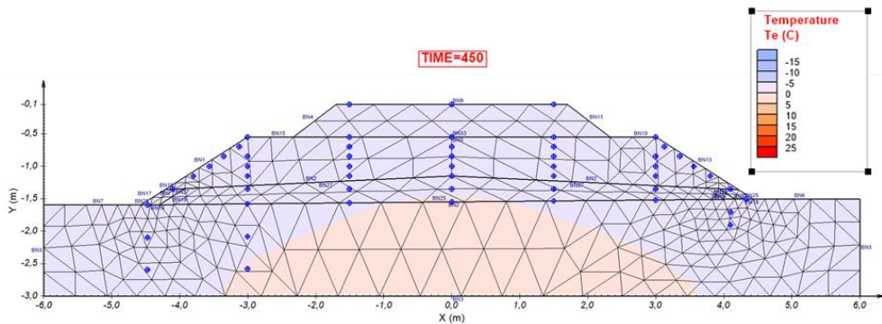
Fig. 6. Graphical output of modeling of the railway track freezing for limit (most adverse winter) boundary climatic conditions ( I_F = -800 °C, day, \theta_m = 5 °C, t_{snow} = 0.25 m)
