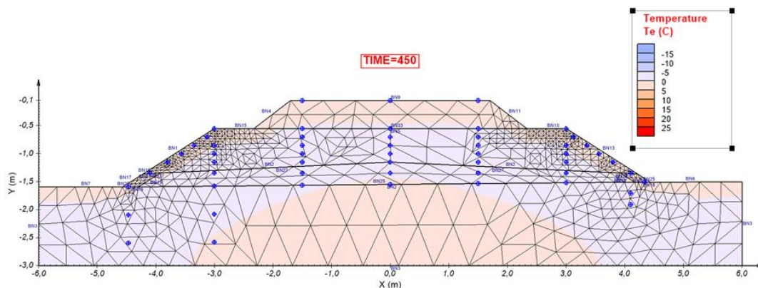
Fig. 4. Graphical output of modeling the railway track freezing for limit boundary climatic conditions ( I_F = -800 °C, day, \theta_m = 5 °C, nf = 0.55 )
