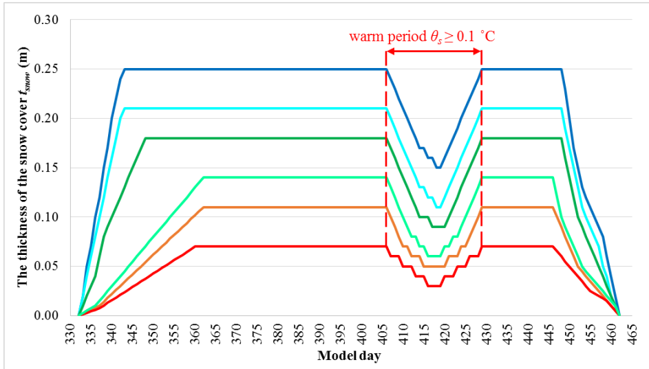
Fig. 7. Considered values of snow cover thickness in a numerical model
