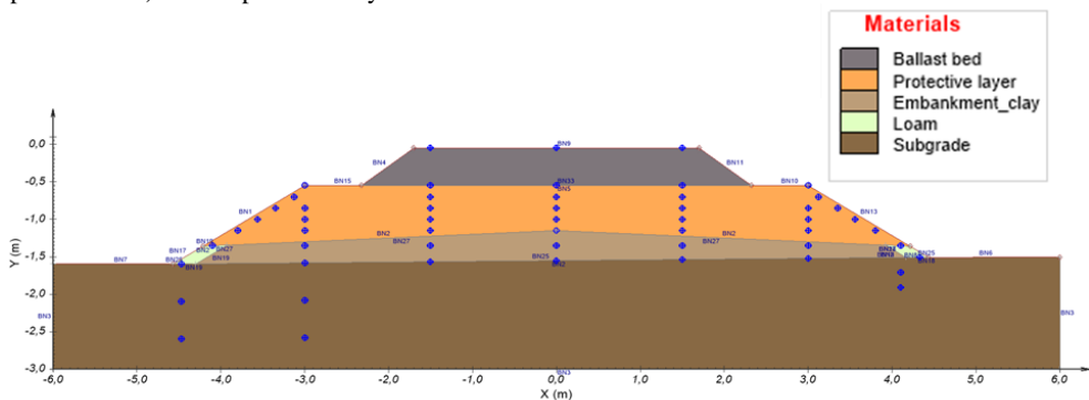
Fig. 1. Model of the Experimental stand DRETM – measuring profile No.1
