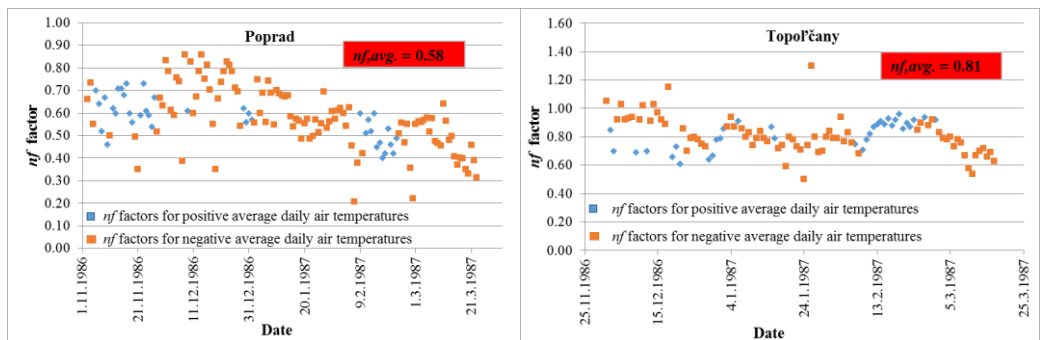
Fig. 2. Stated nf factor values for winter period 1986/87 (left – meteorological station Poprad, right – meteorological station Topoľčany)
