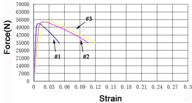
Fig. 2. Force-strain curve of 18Ni (250)
