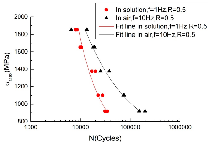
Fig. 5. S-N curve curves (survival probability P_s = 0.5 ) of 18Ni (250) in air and 3.5% NaCl solution
