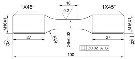
Fig. 3. Sample of axial stress fatigue
