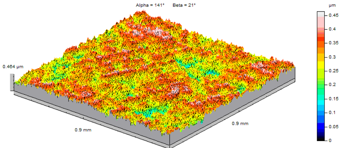
Fig. 3. Isometric picture (3D) of the surface of the stainless steel substrate
