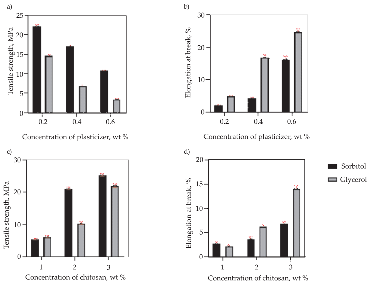
Fig. 2. a) Tensile strength, b) elongation at break of Gracilaria sp.-based thin film + plasticizer, c) tensile strength, d) elongation at break of Gracilaria sp.-based thin film + plasticizer + chitosan
