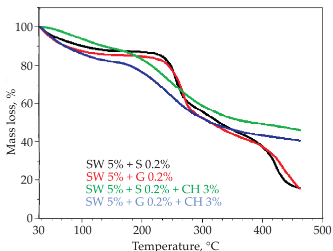
Fig. 4. TGA graph of Gracilaria sp.-based thin film
