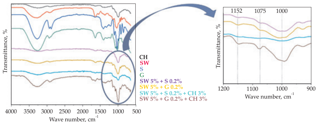
Fig. 1. FT-IR spectra of Gracilaria sp.-based thin films
