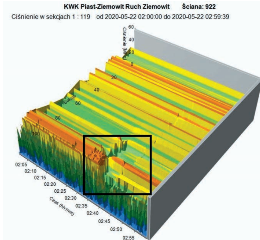
Fig. 15. Side view of the 3D plot of wall 922 – location of the shock
