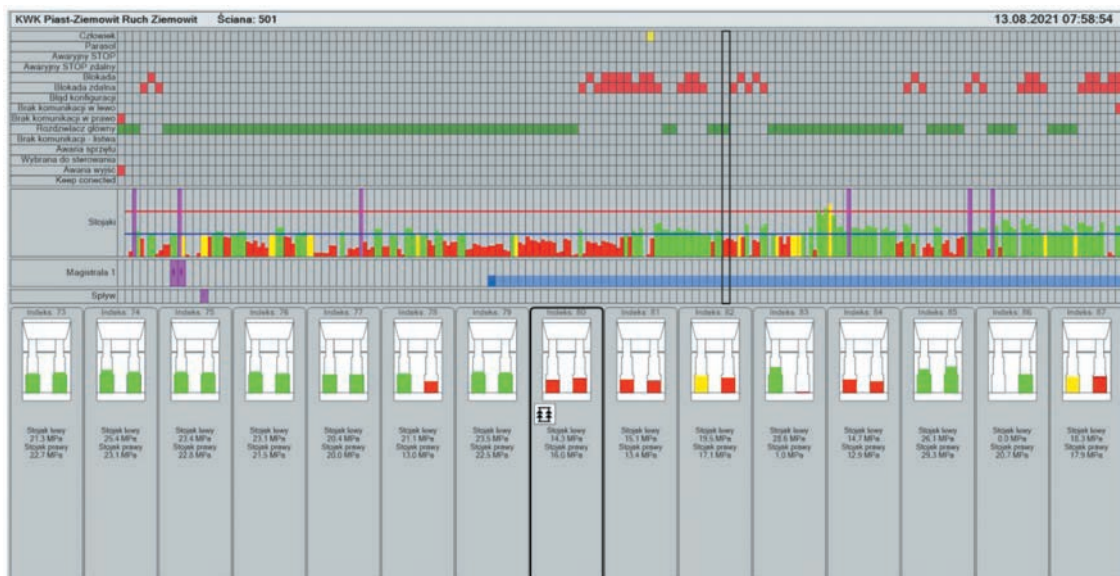
Fig. 5. The state of support in the longwall 501 without the active system applied
