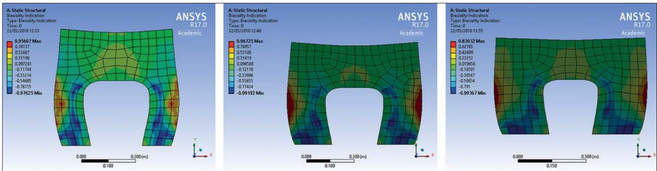
Fig. 19. Distribution of biaxiality indication for specimen 1 and each of the values of the longitudinal spacing (400, 500, and 600 mm)
