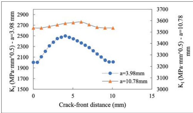
Fig. 25. Stress intensity factor variation on the crack-front in specimen 1
