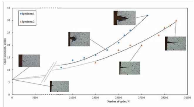
Fig. 21. Evolution of crack length (a) for the number of cycles for both specimens
