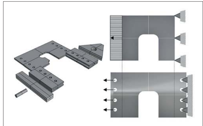
Fig. 7. (left) Arrangement of transition pieces for adaptation and coupling to the testing machine.(right) Comparison between initial and adapted geometry
