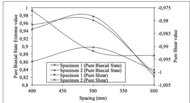
Fig. 20. Pure biaxial state and pure shear for both specimens
