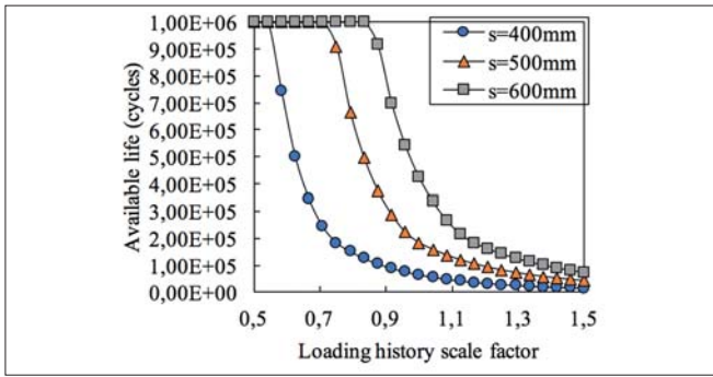
Fig. 18. Fatigue sensitivity curves for specimen 1
