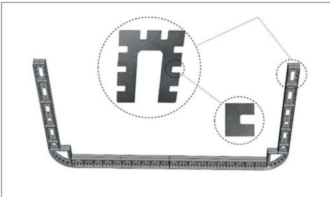
Fig. 1. Midship section of the container ship with an upper wing torsional box and cut-out detail
