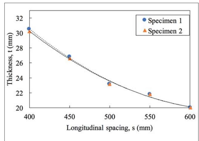
Fig. 17. Relationship between thickness and longitudinal spacing variables using local quadratic regression model for both specimens
