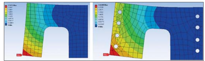
Fig. 10. Comparison between both geometries when determining the value of the maximum displacement of specimen 1
