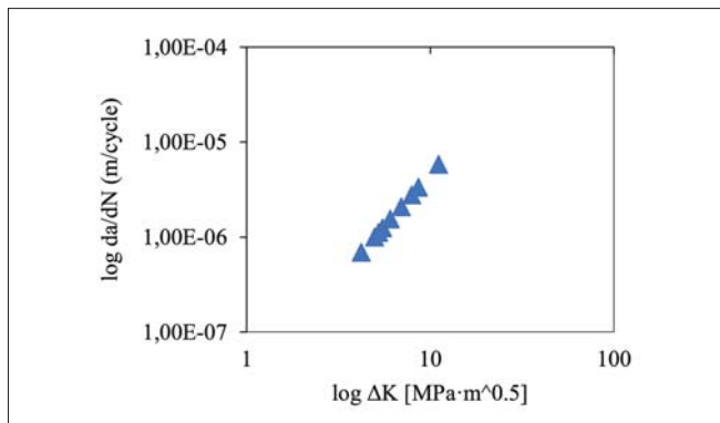
Fig. 22. Relationship between crack propagation rate and stress intensity factor range
