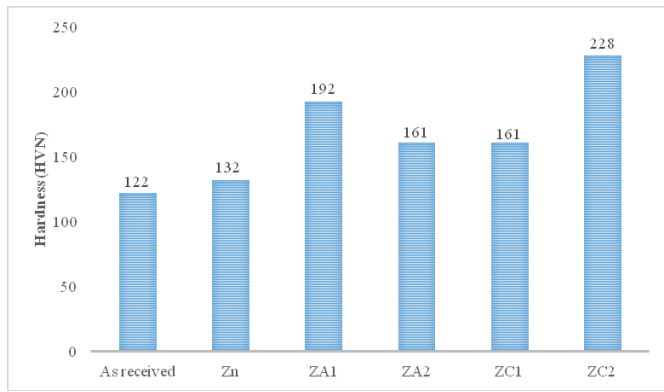
Fig. 6. Microhardness values for as received, Zn, ZA and ZC nanocomposite coatings
