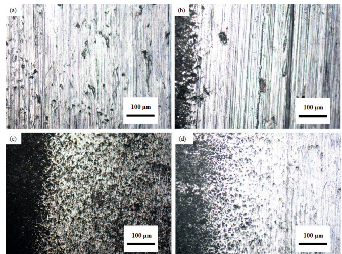
Fig. 11. Optical Microscope micrographs of worn out surfaces (a) as received sample, (b) Zn electrodeposits (c) ZA1 alloy and (d) ZC2 nanocomposite alloy
