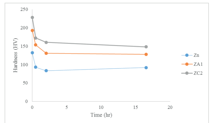
Fig. 8. Variation of microhardness of Zn, ZA1 and ZC2 deposits at 250°C for 0.5, 2 and 16 h.
