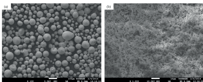
Fig. 1. SEM image of received (a) \text{Al}_2\text{O}_3 and (b) \text{Cr}_2\text{O}_3 powders
