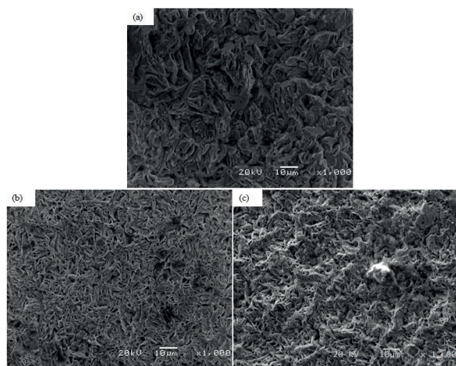
Fig. 2. SEM micrographs (a) Zn coating (b) Zn-5g/L \text{Al}_2\text{O}_3 coating and (c) Zn-20g/L \text{Cr}_2\text{O}_3 coating
