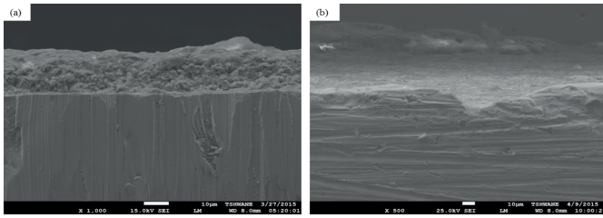
Fig. 3. SEM images of the cross section (a) ZA1 and (b) ZC2 nanocomposite coatings
