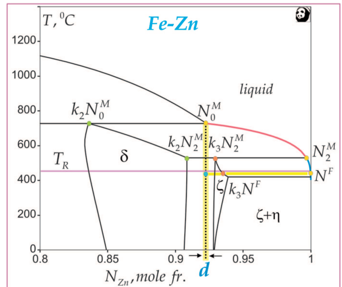
Fig. 6. Fe-Zn phase diagram for meta-stable equilibrium calculated due to the data delivered in Ref. [15], ( Pandat Software ); the red liquidus lines corresponds with the \delta – phase sub-layer formation due to the partitioning which is completed by the undercooled peritectic reaction: \delta(k_2 N_2^M) + liquid(N_2^M) \rightarrow \zeta(k_3 N_2^M) ; the blue liquidus lines corresponds with the \zeta – phase sub-layer formation by the partitioning; N^F \div N_0^M is the dissolution path (yellow line); d(N_0^M) is the localization of the dissolution zone in the phase diagram
