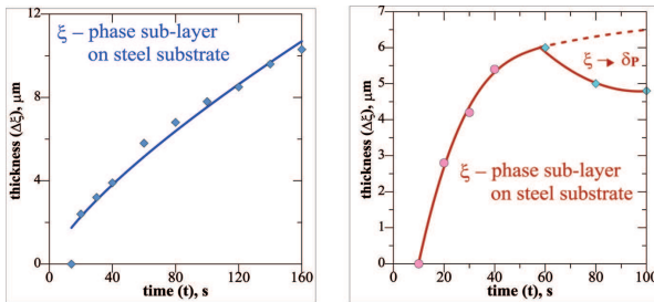
Fig. 12. Tendency of the \zeta – phase sub-layer thickening in the (Zn) – coating settled on: a/ the S235 – steel substrate, b/ the S355 – steel substrate
