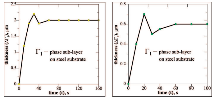
Fig. 3. Tendency of the \Gamma_1 – phase sub-layer thickening/thinning for; a/ the S235 – steel substrate; b/ the S355 – steel substrate
