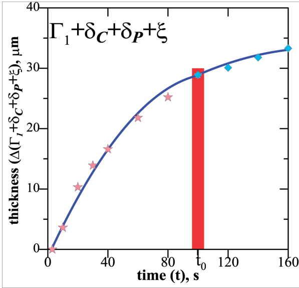
Fig. 16. Kinetics of the \Gamma_1 , \delta_C , \delta_P and \zeta – phase sub-layers growth in the (Zn) – coating settled on the S235 – steel substrate
