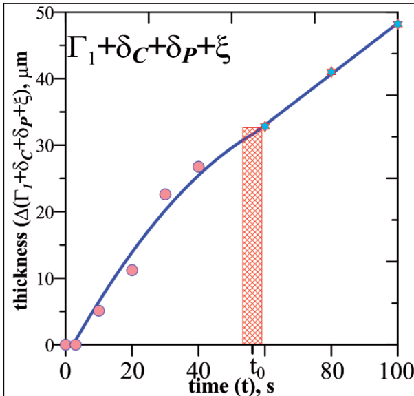
Fig. 17. Kinetics of the \Gamma_1 , \delta_C , \delta_P and \zeta – phase sub-layers growth in the (Zn) – coating settled on the S355 – steel substrate
