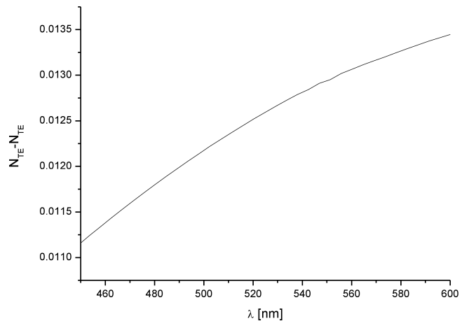
Fig. 6. Dependence of the difference of the effective refractive indices as a function of the wavelength
