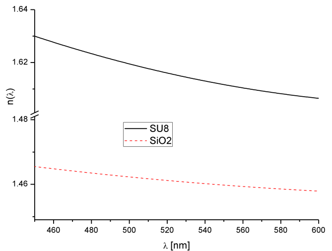
Fig. 3. Spectral characteristics of the refractive indices
