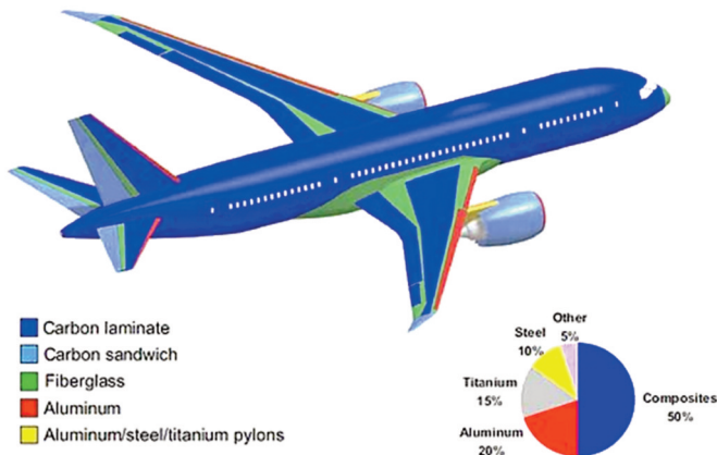
Figure 3. Materials used in Boeing 787 [26]
