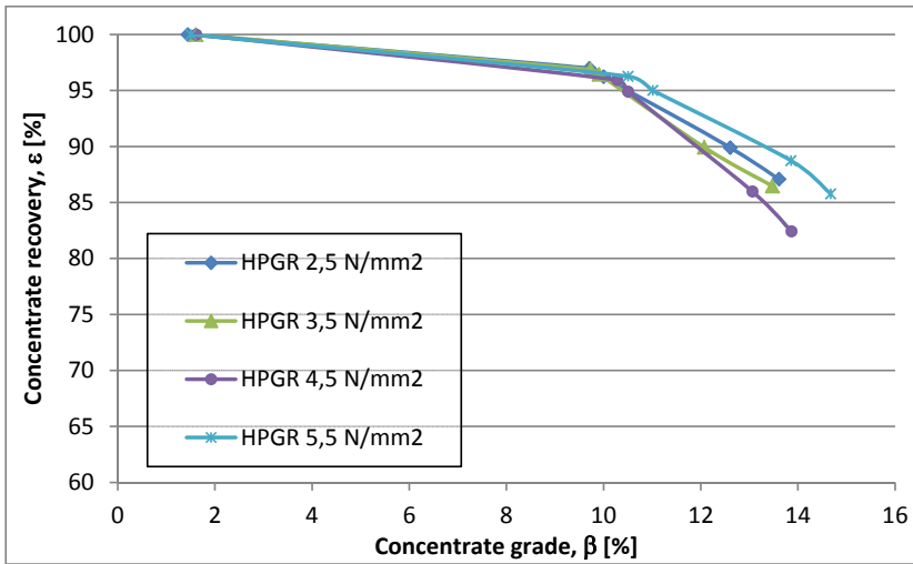
Fig. 6. Halbich upgrading curve for moist material
