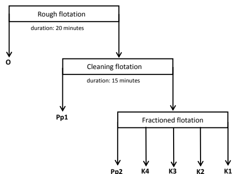
Fig. 3. Diagram of flotation experiment
