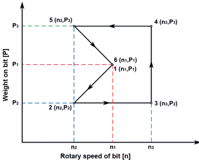
Fig. 2. Scheme of drillability test
