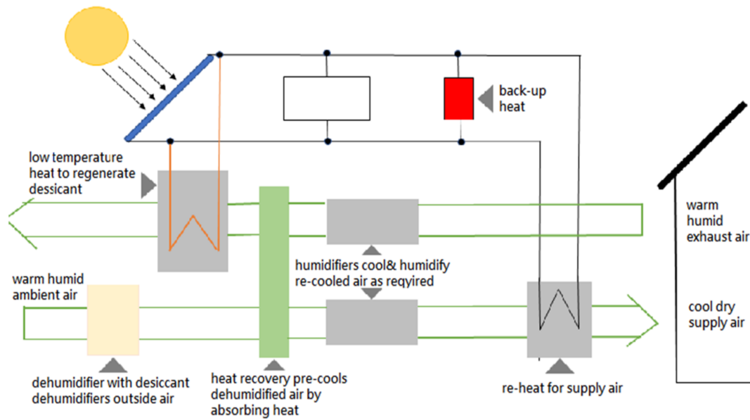
Figure 2. Desiccant cooling system [2].
