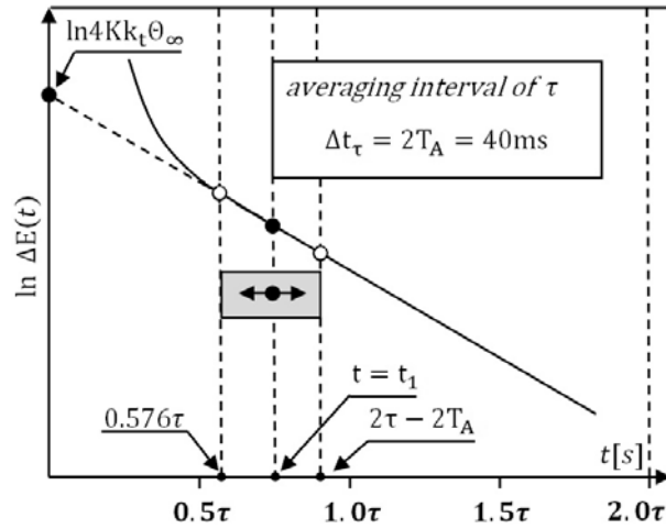
Figure 7. Method for determining the changes of the mean characteristic time \tau(t_1) in the interval (t_2 - t_1) = 40 ms.
