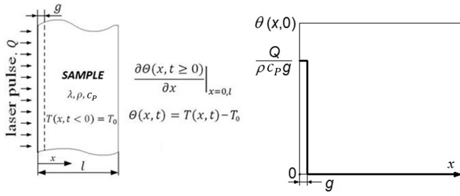
Figure 1. Heat transfer model used for thermal diffusivity of solids determined with the classical and the modified pulse methods.
