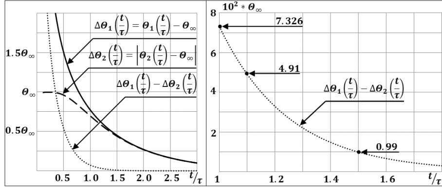
Figure 5. Temperature changes on the boundary surfaces of the specimen \Delta\theta_1(t/\tau) and \Delta\theta_2(t/\tau) referred to \theta_\infty , and their difference.
