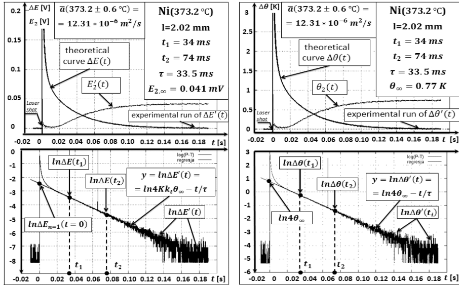
Figure 11. Thermal diffusivity results for Ni (99.9% wt) at the temperature of T = 373.2 \text{ }^\circ\text{C} , and runs of the temperature changes \Theta_2(t) and \Delta\Theta(t) .
