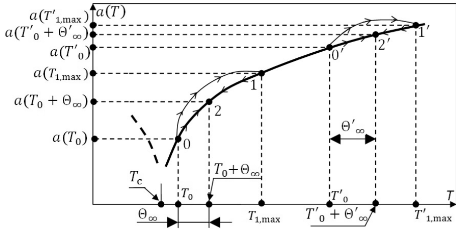
Figure 9. Relative positions of T_0 , and \Theta_\infty , T'_0 , T_C and \Theta'_\infty , and the corresponding values of a(T) .
