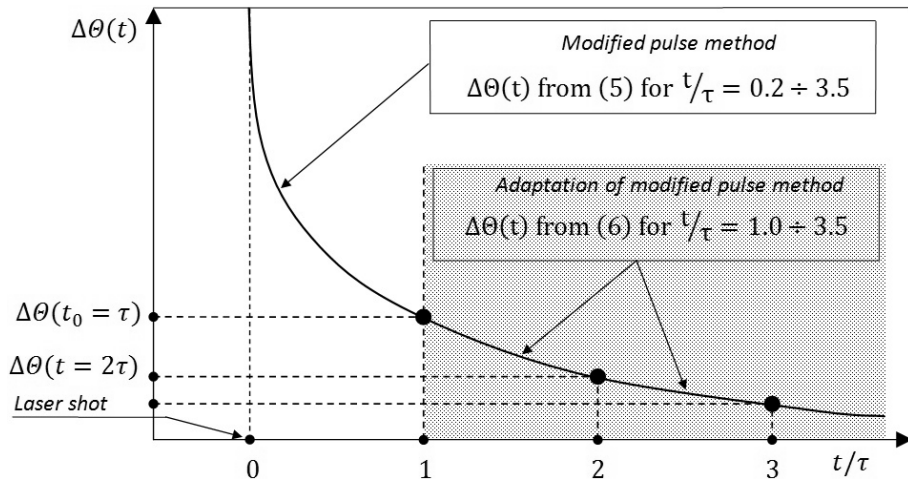
Figure 3. The course of changes of the temperature difference \Delta\theta(t) between the boundary surfaces of the specimen, used for the determination of thermal diffusivity with the modified pulse method, and the section of this course \Delta\theta_{n=1}(t) used after the adaptation of the method.
