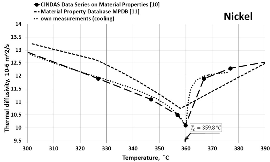
Figure 13. Thermal diffusivity results for Ni with the phase transition taken into account.
