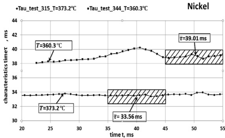
Figure 8. Method for determining characteristic time, \tau , for two temperature values T = 360.3^\circ\text{C} > T_C and T = 373.2^\circ\text{C} > T_C , and when \Delta t_\tau = 40 ms.
