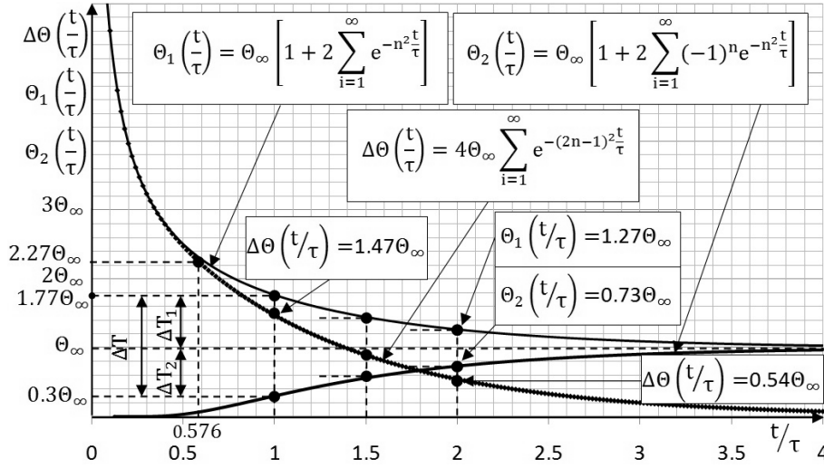
Figure 2. Temperature changes on the boundary surfaces of the investigated specimen and the difference between them with the values characteristic of those changes.
