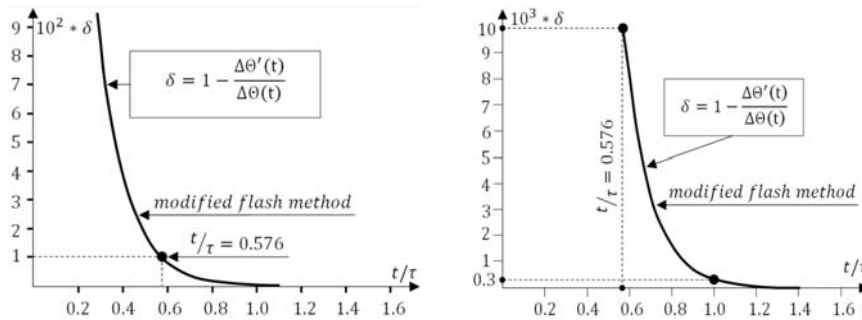
Figure 4. Error \delta(t/\tau) on account of replacing expression (5) for the change of the temperature difference \Delta\theta(t) on the boundary surfaces of the specimen with its approximated form (6).
