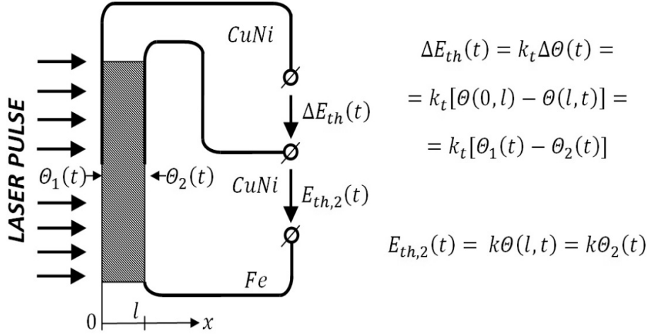
Figure 6. Principle of the sample temperature measurement, \Theta_2(t) , and the difference of the temperature \Delta\Theta(t) between the extreme surfaces of the sample: k_t – the thermoelectric power of the thermocouple ‘CuNi - the material of the investigated sample’; k – the known thermoelectric power of the thermocouple ‘Fe–CuNi’.
