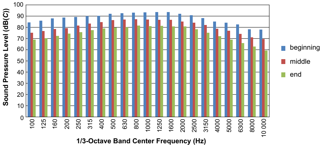
Figure 2. Noise spectrum generated by a continuous mining machine in average working conditions with the double-strand chain conveyor swung to the right.
