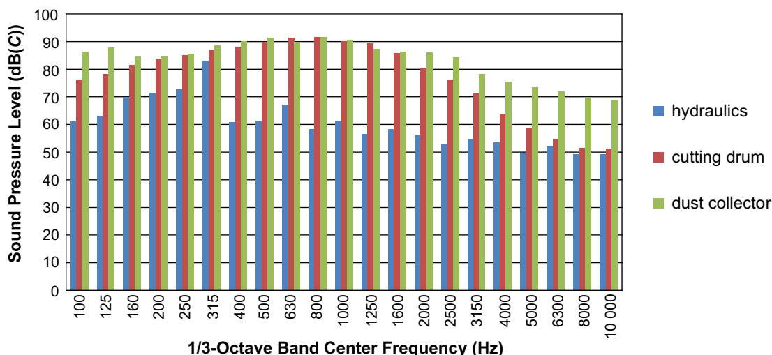
Figure 4. Noise spectrum generated by a hydraulic system, a cutting drum, and a dust collector with a continuous mining machine not mining coal.
