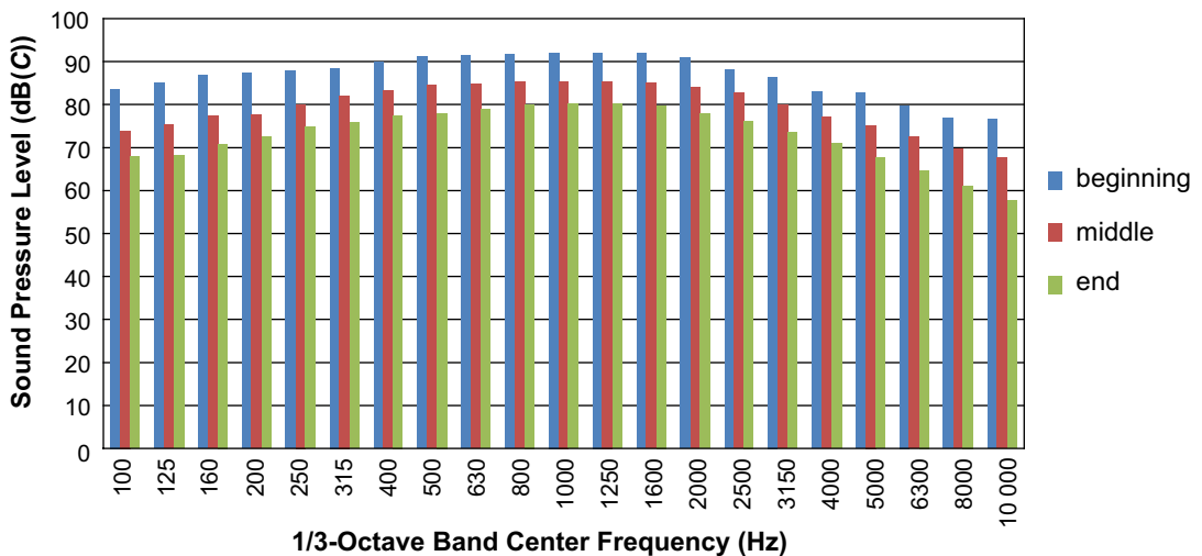
Figure 3. Noise spectrum generated by a continuous mining machine in average working conditions with the double-strand chain conveyor swung to the left.
