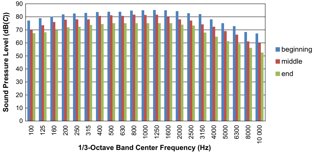
Figure 1. Noise spectrum generated by a continuous mining machine in average working conditions with the double-strand chain conveyor in a straight position.
