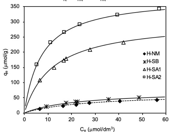
Fig. 3. Adsorption isotherms of Direct Orange 26 from aqueous solution on the halloysites
