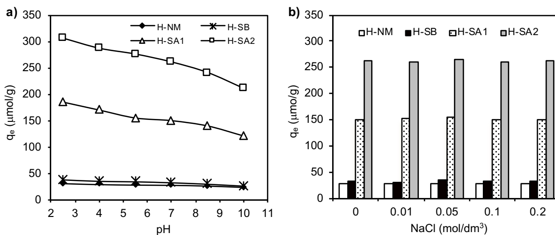
Fig. 4. Effects of initial solution pH (a) and solution ionic strength (b) on adsorption of Direct Orange 26 on the halloysite samples
