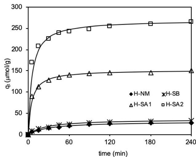
Fig. 2. Adsorption kinetics of Direct Orange 26 on the halloysites
