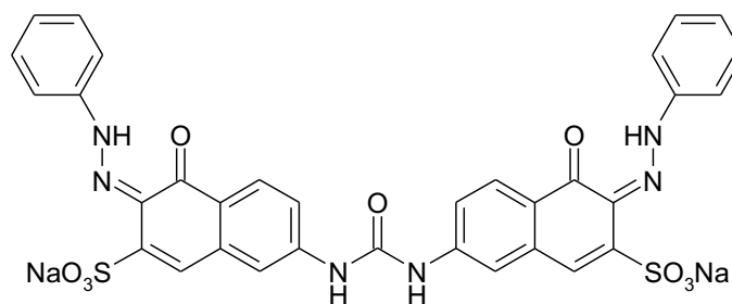
Fig. 1. Chemical structure of Direct Orange 26 azo dye
