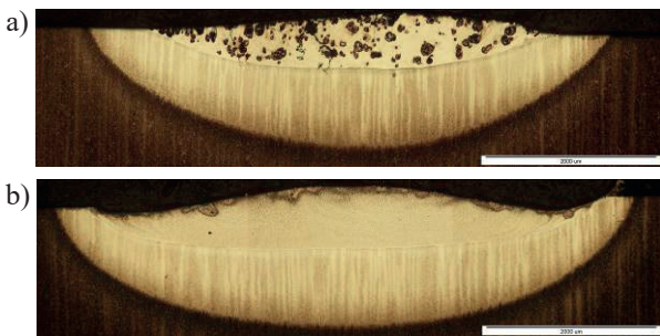
Fig. 5. The cross - section of laser surface alloyed X40CrMoV5-1 steel after laser alloying with a) WC powder and b) VC powder at laser beam power of 2.3 kW
