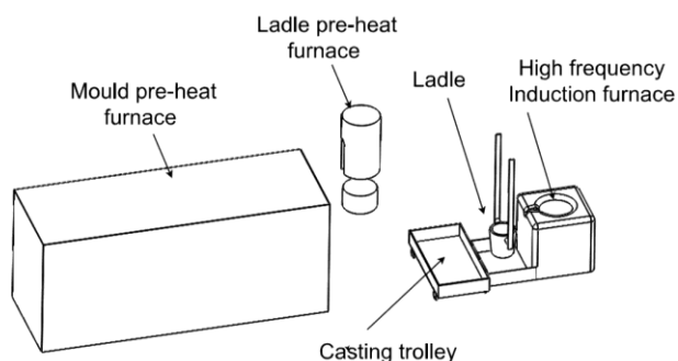
Fig. 1. Casting furnace and set-up for evaluating effects of variations originating from casting practice
