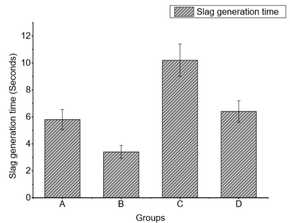
Fig. 6. Slag generation time for different groups
