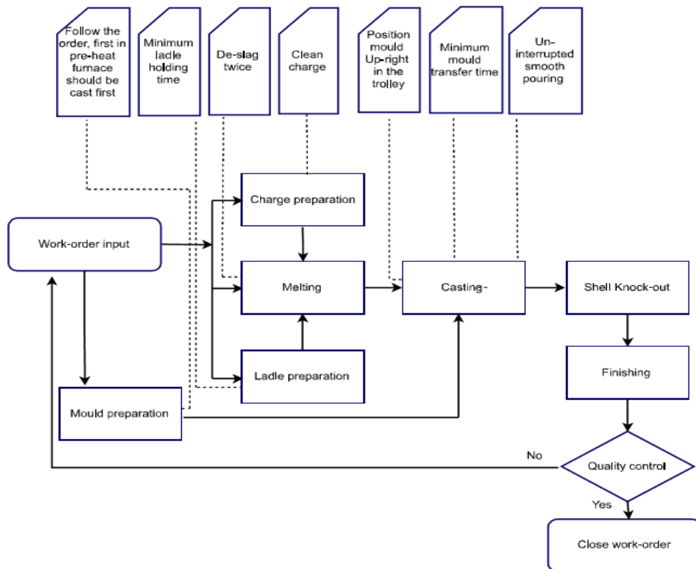
Fig. 9. Instruction card for casting operation at HF induction furnace
