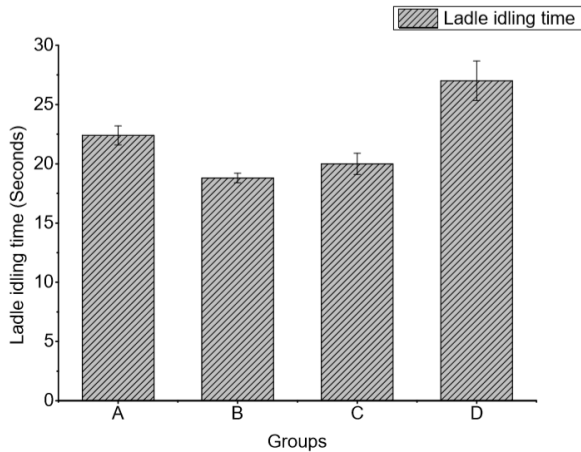
Fig. 2. Ladle idling time for different groups
