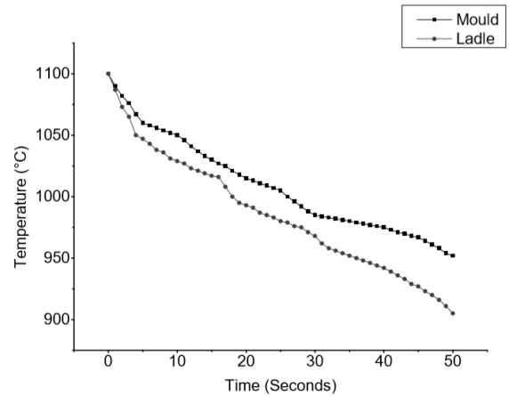
Fig. 5. Temperature drop in the mould and ladle during transportation
