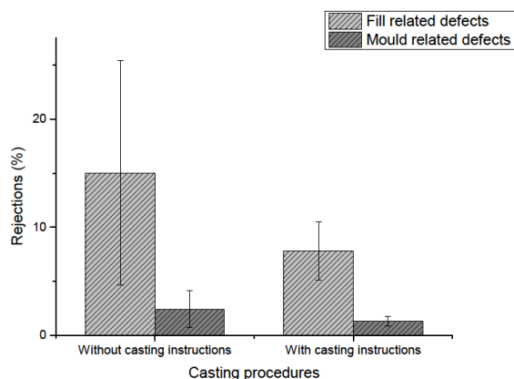
Fig. 10. Rejection percentage before and after implementation of casting instructions presented in Figure 9
