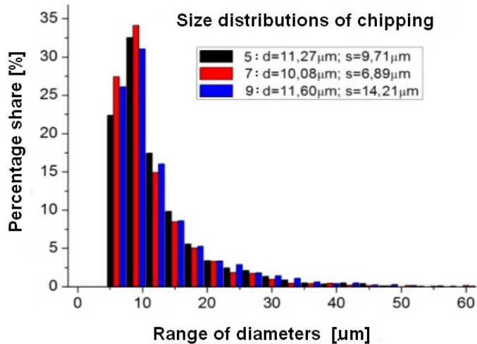
Fig. 6. The size distribution of the areas of crushed out elements of microstructure in the samples of the tested material, which were loaded up to 275, 504 and 582 MPa. The average value is equal to 11 \mu\text{m} (d denotes mean value, s – standard deviation for the particular sample)
