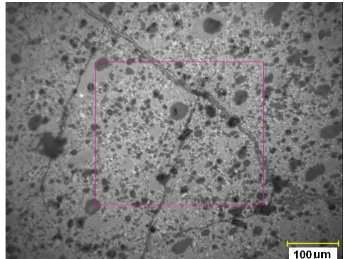
Fig. 7. The cracking system in the middle part of the sample of the tested material, subjected to destruction at 690 MPa, \times 200 . There are numerous dark areas after crushed out elements of the microstructure – particles of cullet, quartz, mullite precipitates and corundum agglomerates. They constitute a total of 22% of the surface area
