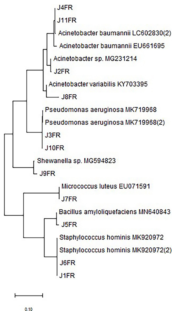
Figure 5. Phylogenetic tree
