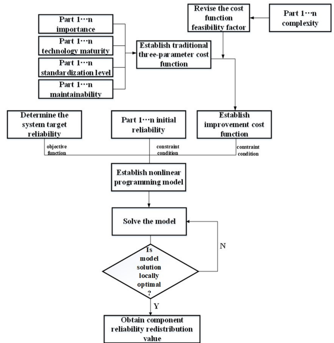
Fig. 6. Algorithm flow chart of reliability optimization allocation method based on improved cost function
