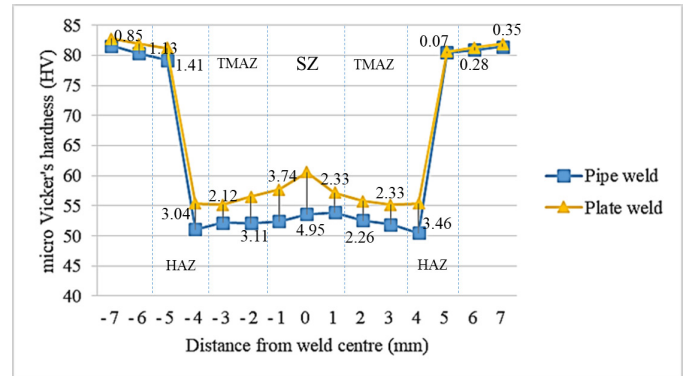
Fig. 5. Results of Hardness test (with standard deviation)
