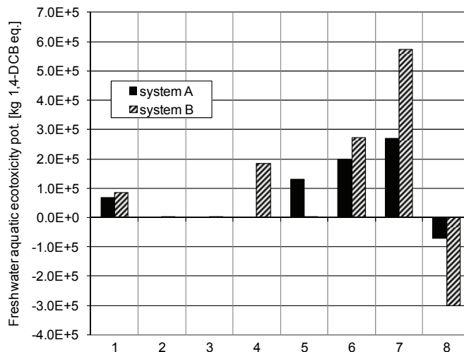
Fig. 5. Freshwater aquatic ecotoxicity of two Cracow MSWM systems 1 – collection, 2 – sorting, 3 – biological treatment, 4 – thermal treatment 5 – landfill, 6 – IWM model total, 7 – recycling savings, 8 – overall total
