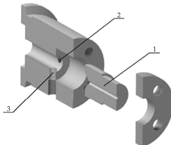
Fig. 1. Rheological extrusion head: 1 – exchangeable cylindrical die, 2 – thermocouple, 3 – pressure sensor
