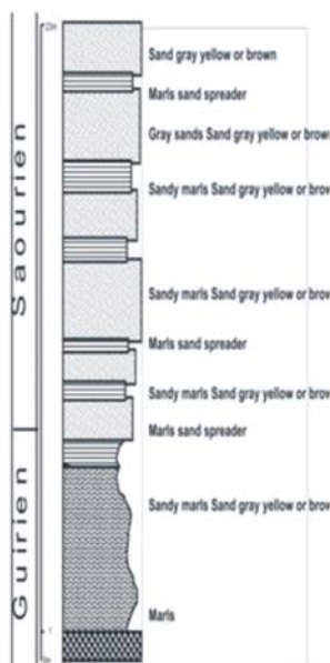
Fig. 3. Quaternary diagrammatic cross; source: ROCHE [1973]
