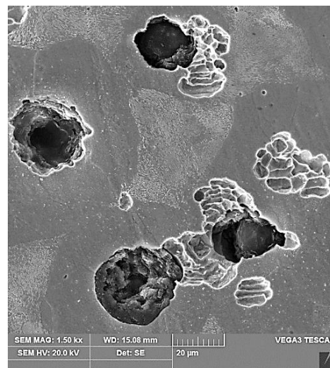
Fig. 6. The second stage of cast iron microstructure degradation. An outermost portion of cavitation interaction spot. Note high degree of graphite precipitate degradations progressing in layers but always from center towards graphite-matrix interface. Partial graphite tear-offs initiate degradation of ferritic matrix
