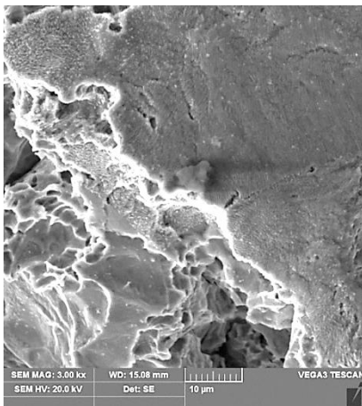
Fig. 8. The second stage of cast iron microstructure degradation. A central portion of the cavitation interaction spot. Deep cavitation-induced cavities in ferritic matrix with visible initial stage of destruction of an exposed, deeply lying graphite precipitate. No visible damages to pearlite precipitates
