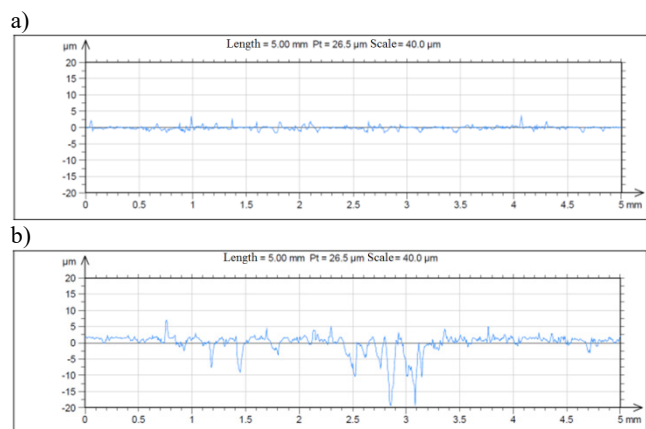
Fig. 3. Example profilograms of nodular cast iron specimen surfaces subject to cavitation erosion test for: (a) 30 minutes, (b) 120 minutes
