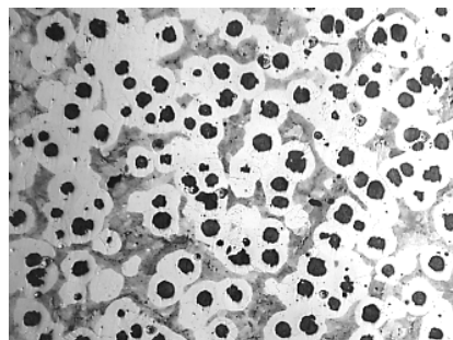
Fig. 2. Microstructure of the nodular cast iron used in the present study. Ferrite, pearlite, graphite. Magnification 100\times . Section etched with 4% \text{HNO}_3
