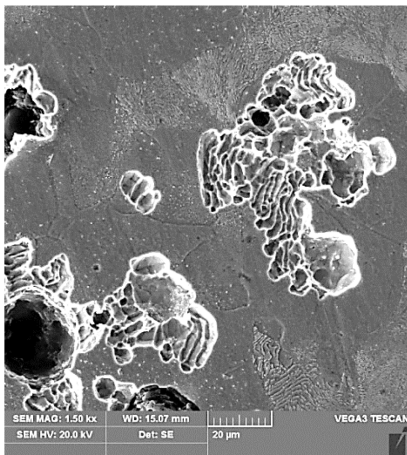
Fig. 7. The second stage of cast iron microstructure degradation. Uttermost region of the cavitation interaction zone. Significant progress in ferritic matrix degradation blocked locally by pearlite precipitation areas
