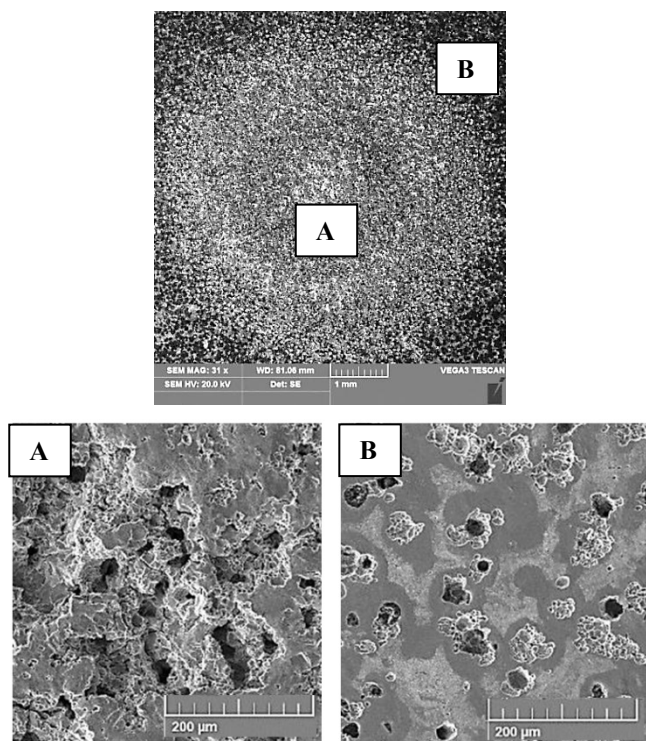
Fig. 4. Example views of specimen surface after 120 minutes of cavitation erosion resistance testing; A — central and B — outermost area of cavitation interaction spot
