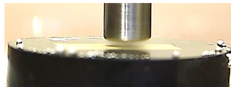
Fig. 1. A view of the cavitation mist area developed over the specimen surface in the course of cavitation erosion test
