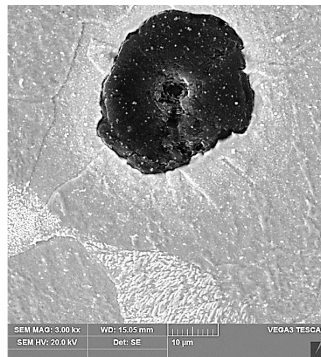
Fig. 5. The first stage of cast iron microstructure degradation. Outermost portion of cavitation interaction spot. Destruction of graphite precipitates in ferritic matrix progressing from center towards graphite-matrix interface
