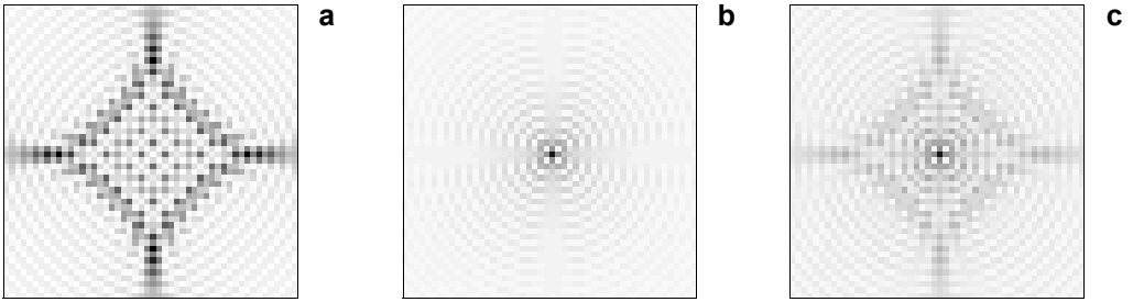
Fig. 4. Calculated intensity distributions (negative images) when the polarization is at 45^\circ to the c -axis ( \varphi_p = 45^\circ , \varphi_c = 0^\circ ): x -component ( \varphi_a = 0^\circ ) – a , y -component ( \varphi_a = 90^\circ ) – b , and total intensity – c .
