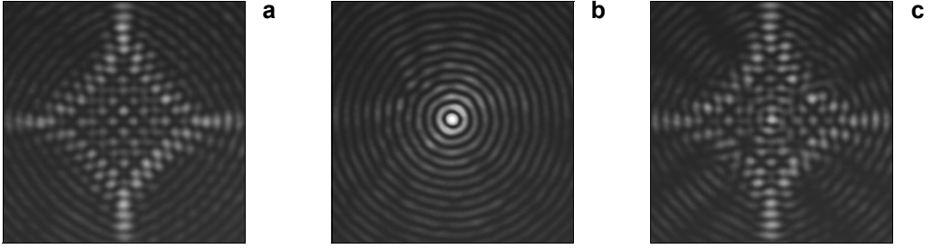
Fig. 8. Experimental intensity distributions when the polarization is at 45^\circ to the c -axis ( \varphi_p = 45^\circ , \varphi_c = 0^\circ ): x -component ( \varphi_a = 0^\circ ) – a , y -component ( \varphi_a = 90^\circ ) – b , and x - and y -component ( \varphi_a = 45^\circ ) – c .
