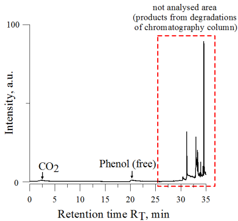
Fig. 2. Chromatogram of sample S1
