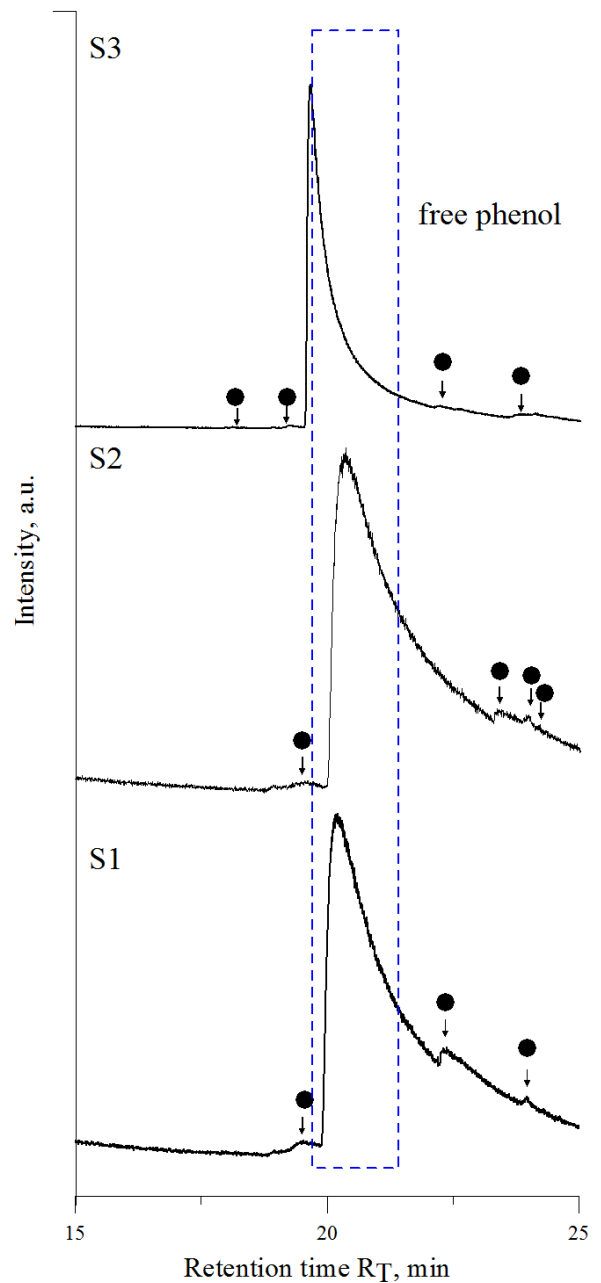
Fig. 5. Chromatograms with marked signal of emission of phenol and its derivatives (black dots)
