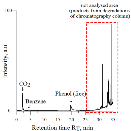
Fig. 4. Chromatogram of sample S3
