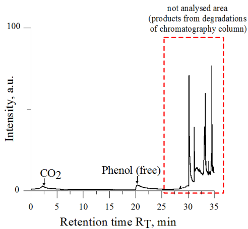
Fig. 3. Chromatogram of sample S2
