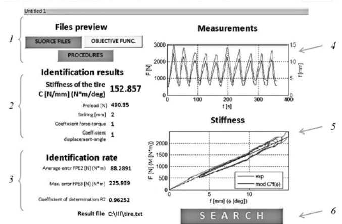
Fig. 3. The dialog box to stiffness identification program (Matlab-Simulink, Guide addition)
