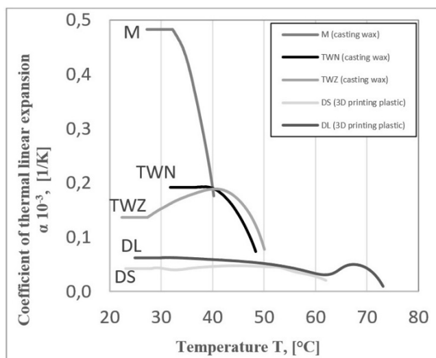
Fig. 2. Changes in the coefficient of thermal linear expansion of foundry pattern materials as a function of temperature
