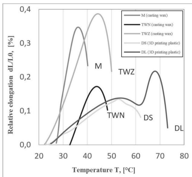
Fig. 1. Changes in relative elongation of foundry pattern materials as a function of temperature
