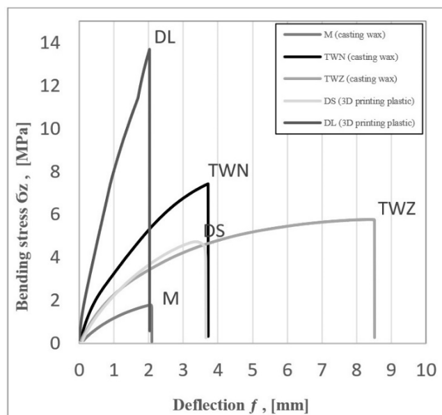
Fig. 3. Bending stress-deflection curves recorded for foundry pattern materials
