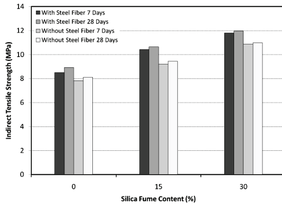
Fig. 11. Indirect tensile strength for samples of 800 kg/m 3 cement content.
