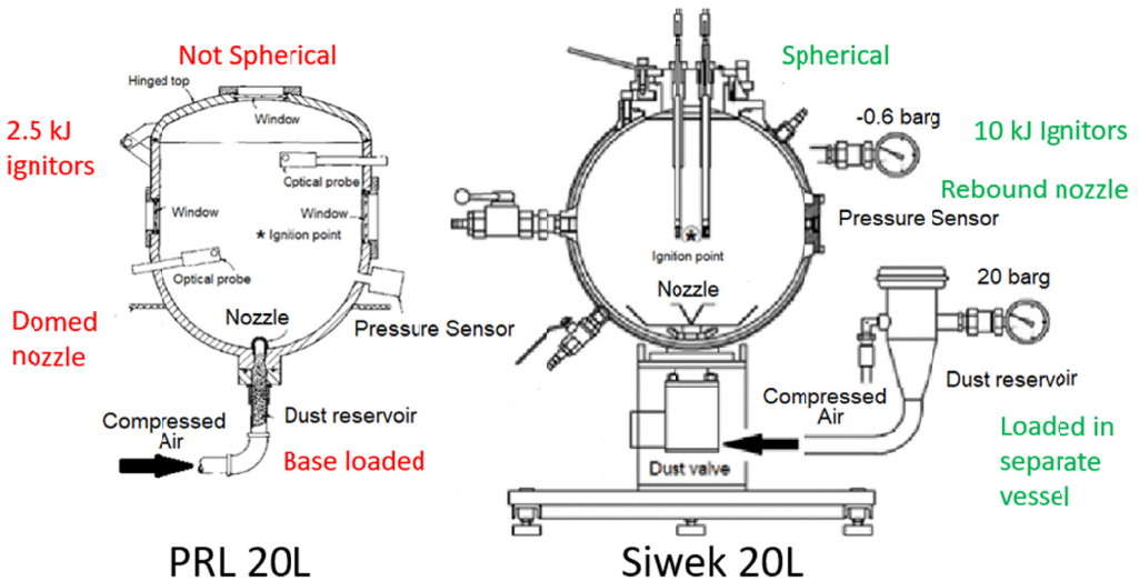
Fig. 3. A Comparison of the USBM PRL 20L on left (adapted from Cashdollar, 1996) and the Siwek 20 Liter on right (adapted from Kuhner AG, 2011)
