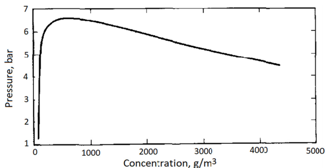
Fig. 2. Expanded Explosibility Data for Pittsburgh Coal Dust, modified from (Cashdollar, 1996)
