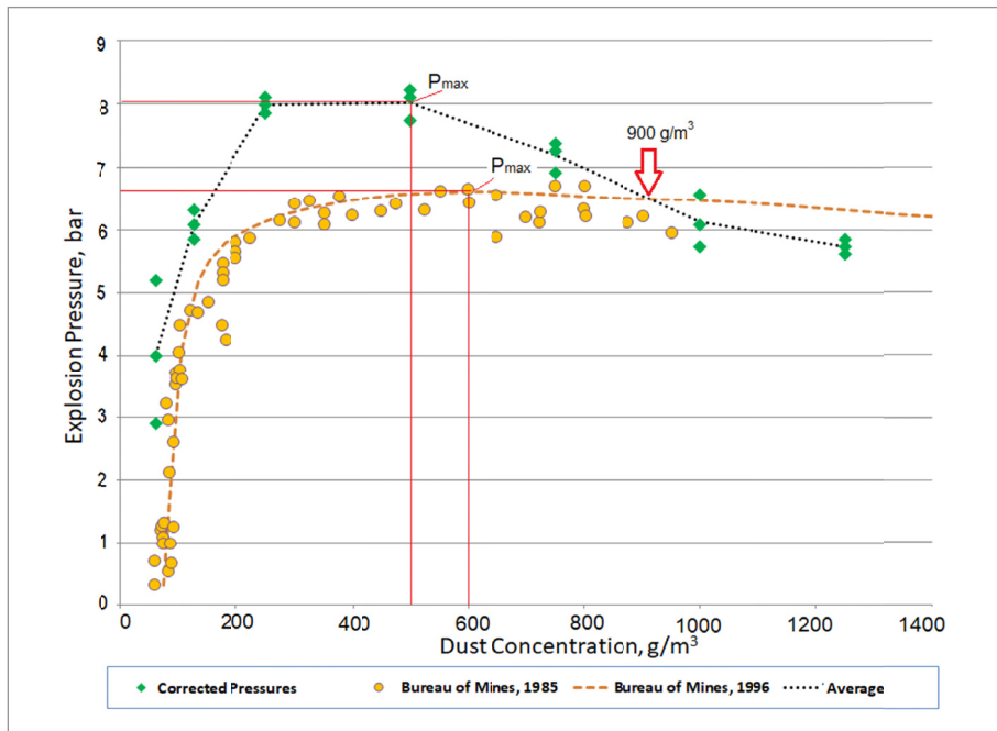
Fig. 6. Explosion Pressure – MS&T Data with Referenced Data (Cashdollar et al., 1985; Cashdollar, 1996)
