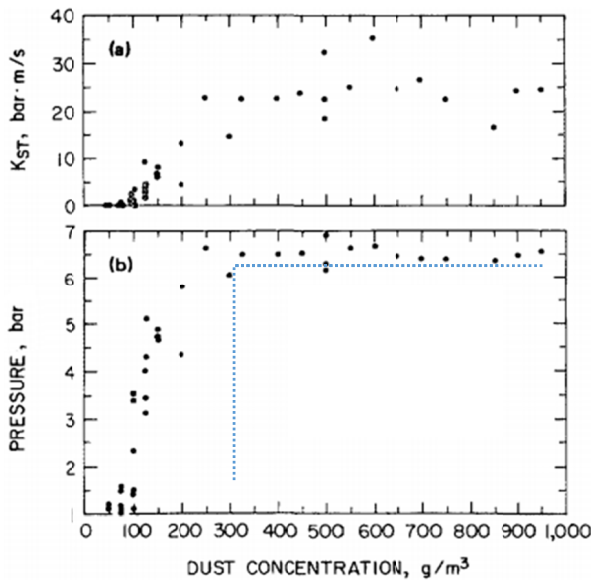
Fig. 1. Explosibility Data for Pittsburgh Coal Dust, modified from (Cashdollar et al., 1985)
