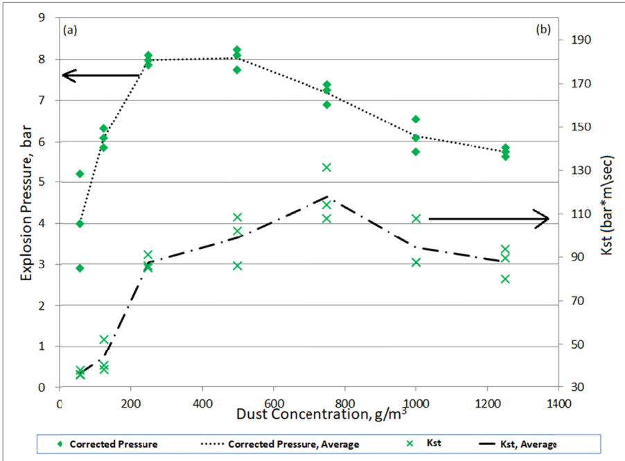
Fig. 5. P_m and K_{st} for PPC dust in University Siwek 20L sphere
