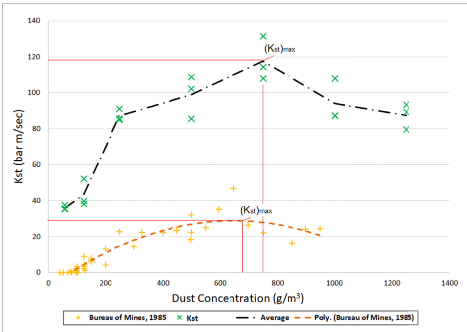
Fig. 7. Explosion KST – University Data with Referenced Data (Cashdollar, 1996)
