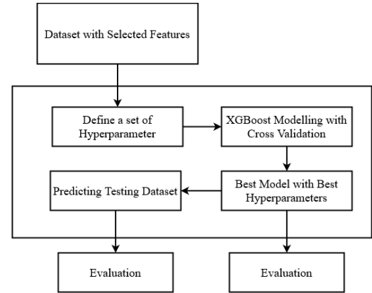
Fig. 4. XGBoost Modeling Flowchart
