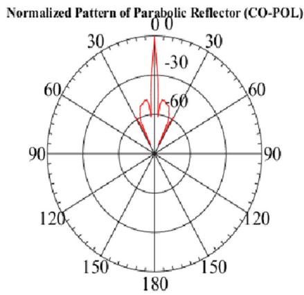
Figure 4. Normalized pattern of reflector
