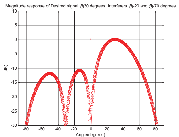
Figure 8. Magnitude response for patch array feed
