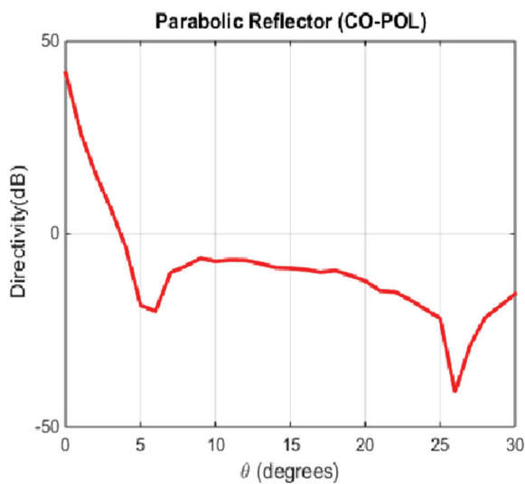
Figure 5. Directivity of the parabolic reflector
