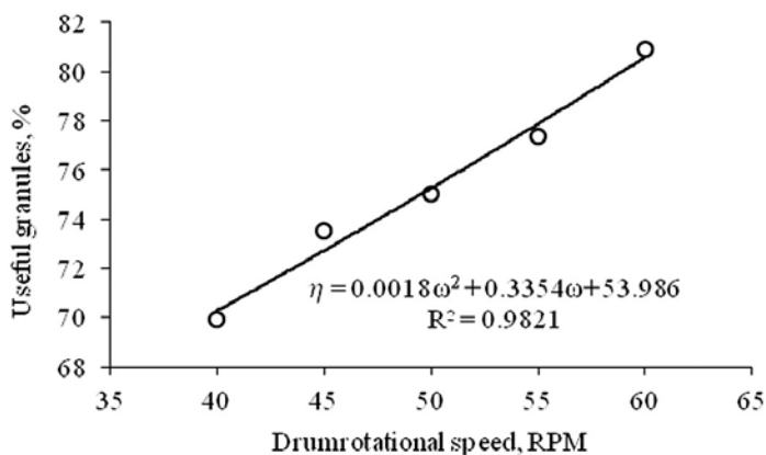
Fig. 3. Effect of drum rotational speed on percentage of useful granules
