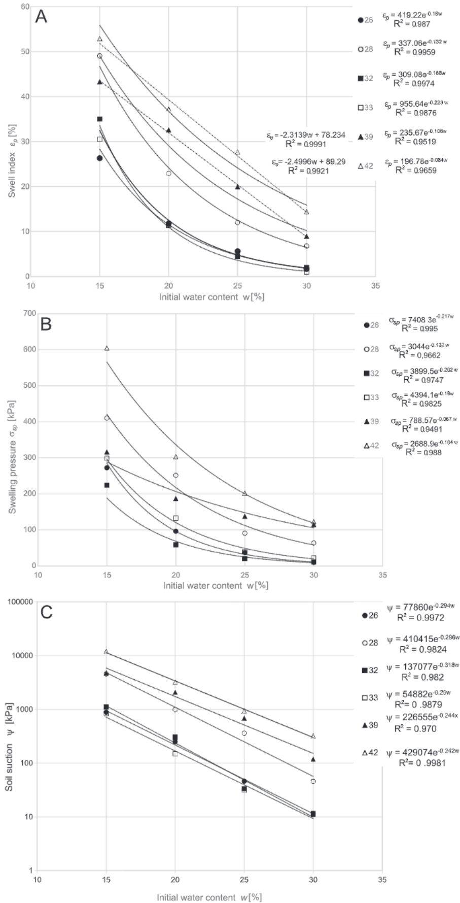
Fig. 5. The effect of initial water content on: A – swell index, B – swelling pressure, C – soil suction
