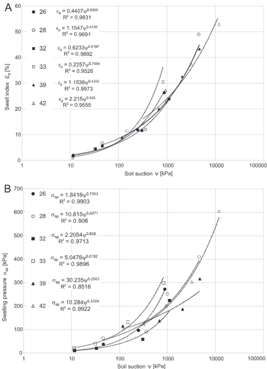
Fig. 6A – the relationship between swell index and soil suction; B – the relationship between swelling pressure and soil suction
