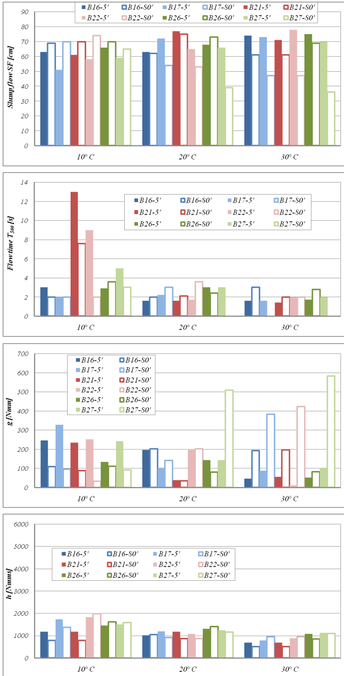
Fig.3. Effect of temperature on workability of self compacting concrete with w/c ratio 0,4.
