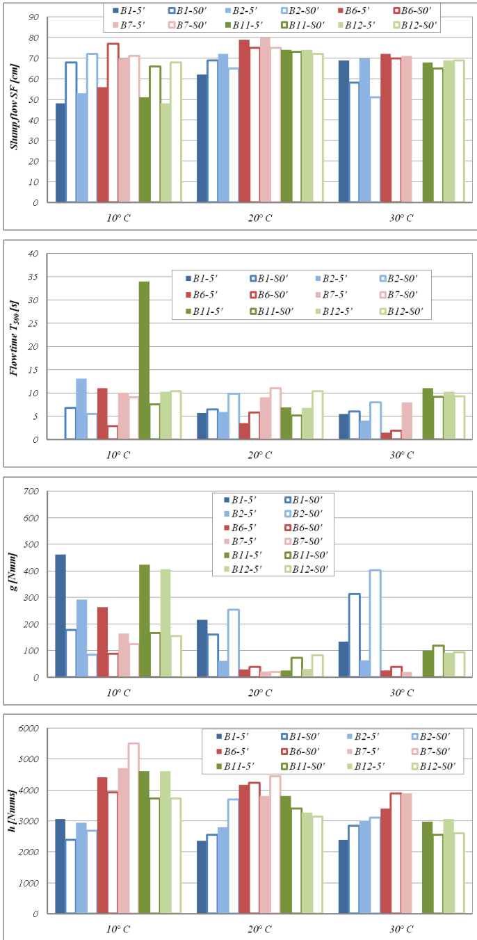
Fig.2. Effect of temperature on workability of self compacting concrete with w/c ratio 0,3.
