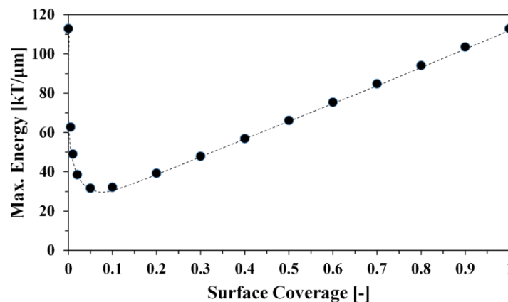
Fig. 5. The effect of particle surface coverage by 5 nm (height) asperities on the maximum value of the total interaction potential for 150 μm hydrophobic particle interacting with a (rigid) gas bubble surface, normalized per particle radius. The parameters used were the same as for Fig. 2
