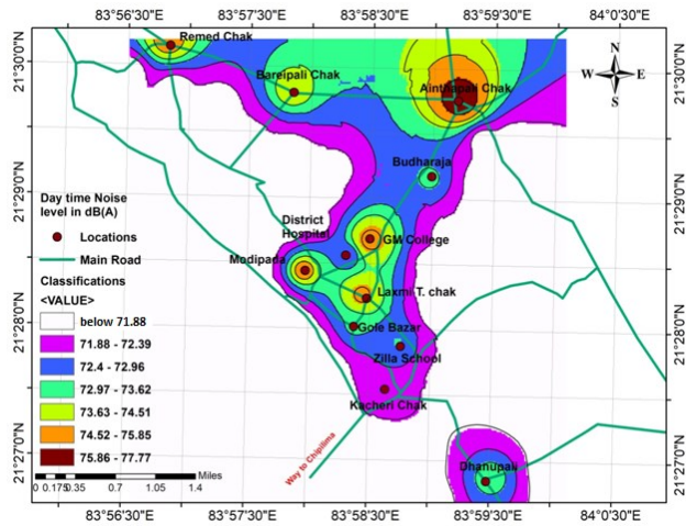
Fig. 10. Noise mapping of the city (due to traffic noise) during day hours.
