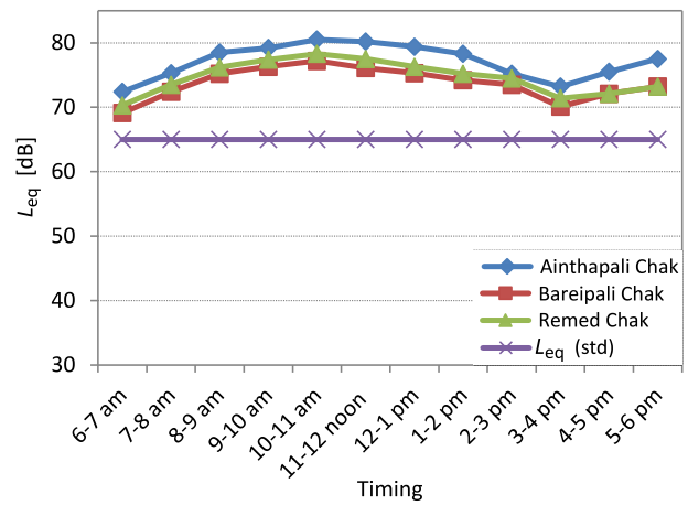
Fig. 8. L_{eq} at different locations (of commercial area on NH) during day hours.
