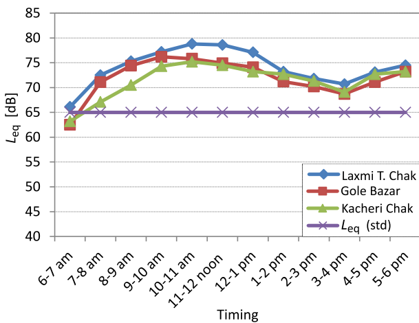
Fig. 6. L_{eq} at different locations (of commercial area) during day hours.
