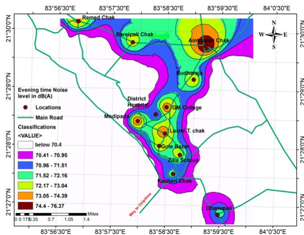
Fig. 11. Noise mapping of the city (due to traffic noise) during evening hours.
