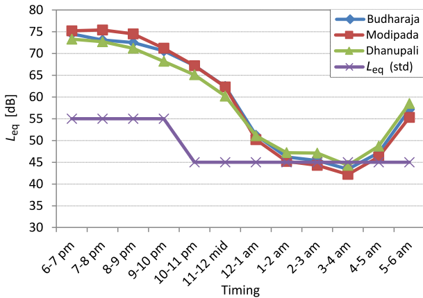
Fig. 5. L_{eq} at different locations (of residential area) during evening-night hours.
