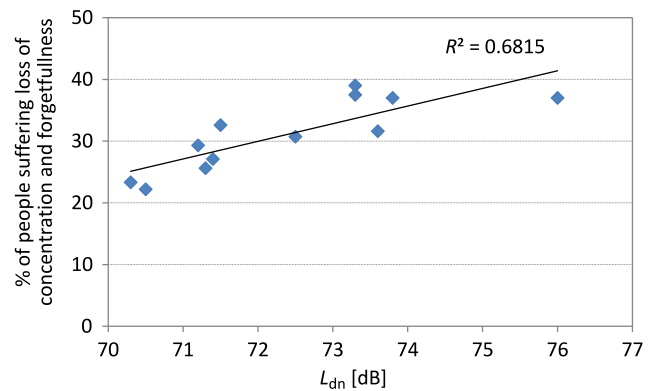
Fig. 14. L_{dn} versus percentage of people suffering from loss of concentration and forgetfulness at different locations.
