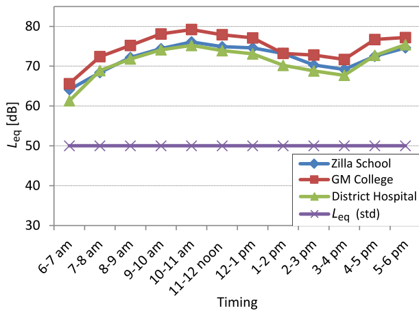
Fig. 2. L_{eq} at different locations (of silent area) during day hours.
