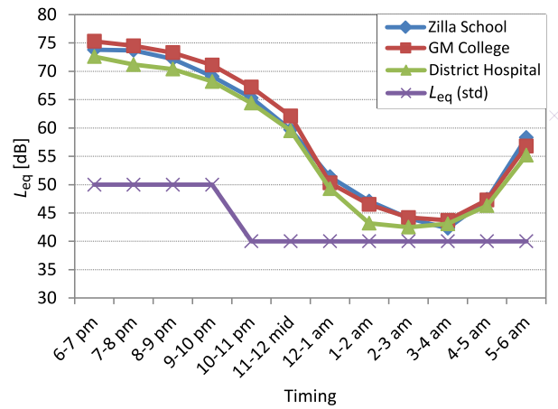
Fig. 3. L_{eq} at different locations (of silent area) during evening-night hours.
