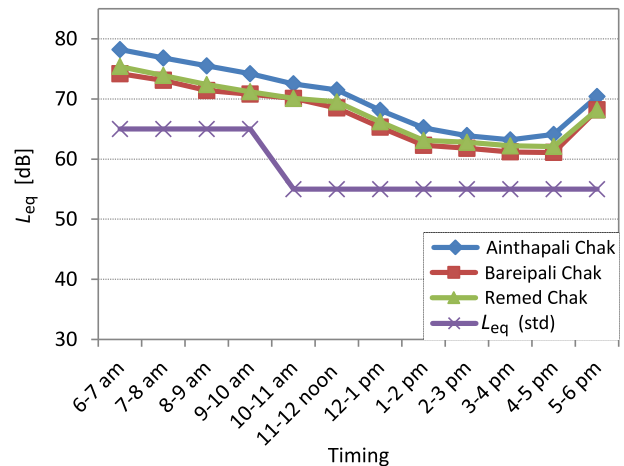
Fig. 9. L_{eq} at different locations (of commercial area on NH) during eve-night hours.
