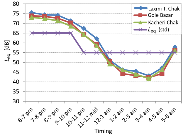
Fig. 7. L_{eq} at different locations (of commercial area) during evening-night hours.
