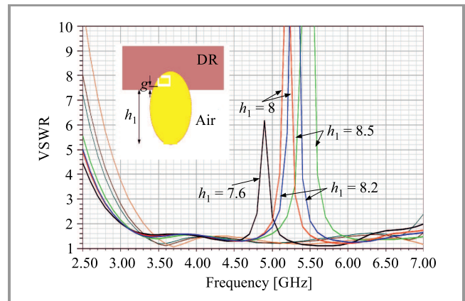
Fig. 9. VSWR characteristics of the single notch band for various h_1 ( L_{slot} = 7.2 \text{ mm} ).
