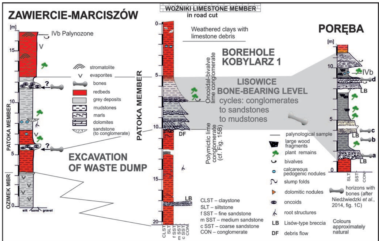
Fig. 14. The lithological section of the Zawiercie-Marciszów site (see Figs 11 and 16), as exposed in the municipal dump excavation in 2000 (reproduced from Budziszewska-Karwowska et al. , 2010, fig. 2, based on Szulc et al. , 2006, fig. 5; modified) and in the Kobylarz 1 well (Szulc et al. , 2015) and at the Poręba site (based on Niedźwiedzki et al. , 2014, fig. 1C and observations of the present authors). Arrows indicate alleged bone-rich horizons of the hypothetically-defined Lisowice level, suspected as a source for material exploited since 2009 in the adjacent mound of the Keuper deposits derived from the dig (see Figs 11, 15, 16).
