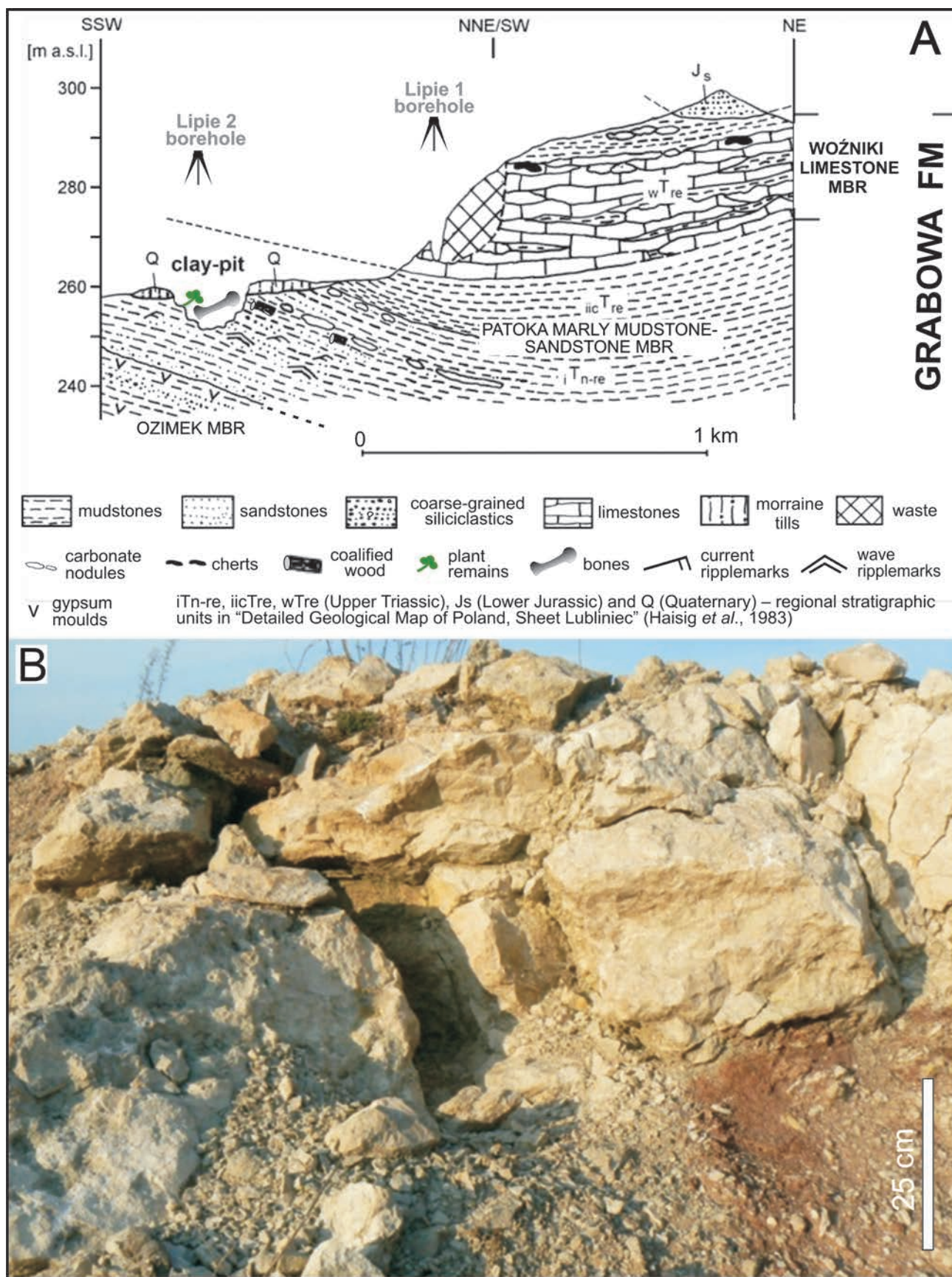
Fig. 7. Schematic geological section across outcrops in the Lisowice - Lipie Śląskie area ( A ; from Bardziński and Chybiors, 2013), and the Woźniki Limestone Mbr above the brown mudstones, mostly covered by a rubbish dump, as recently visible (November 2014) in an inactive quarry on the Lisowice Hill, situated some 400 m N of the pit ( B ; see Figs 5 and 8, compare Szulc et al. , 2006, fig. 8B; see also Gąsiorowski et al. , 1986; courtesy of Waldemar Bardziński).
