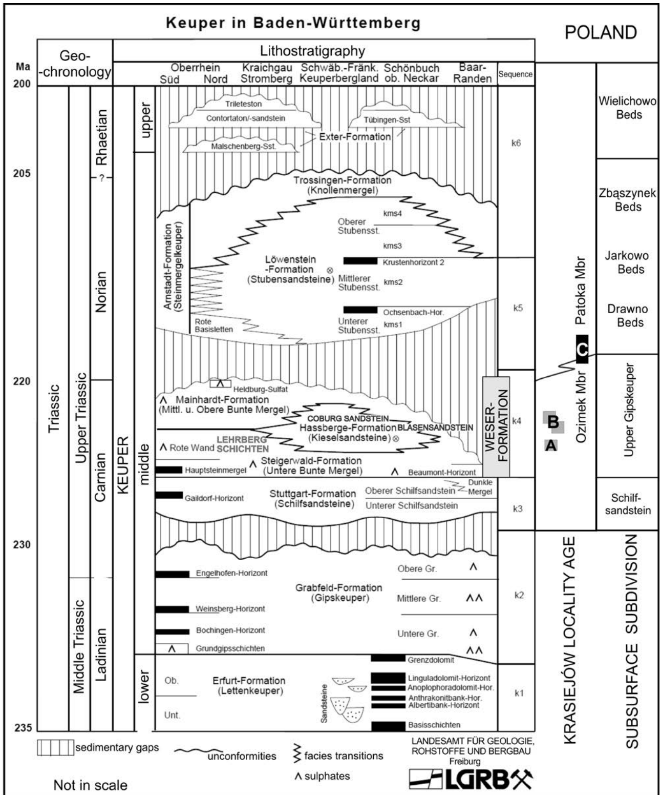
Fig. 4. Three main correlation variants of the Krasiejów clay pit section with the updated reference German Keuper profile (in basin margin facies) of Baden-Württemberg (Nitsch, 2011) and Polish stratigraphic schemes (Dadlez and Kopik, 1963; Becker et al. , 2008; Szulc and Racki, 2015): (A) with the Lehrberg Beds (Steigerwald Fm), based on the original vertebrate evidence of Dzik et al. (2000), favoured, among others, by the inference from conchostracan dating (Kozur and Weems, 2010); (B) with the Blasensandstein or Coburg Sandstein of the Hassberge Fm, supported by revised vertebrate data (Milner and Schoch, 2004; Butler et al. , 2014, fig. 1B) and macrofloral evidence (Pacyna, 2014), respectively; (C) with the Arnstadt Fm, deduced initially from facies development and palynostratigraphic dating (Szulc, 2005, 2007a; cf. also Gruszka and Zieliński, 2008), confirmed by the present, integrative, stratigraphic study (see Fig. 17); the Weser Fm is a lateral equivalent in central basin facies. Note more continuous deposition in Silesia region than assumed in DST 2002 (Szulc et al. , 2015), recorded in the transition from the Upper Gipskeuper to Steinmergel facies at Krasiejów (= Ozimek and Patoka mbrs of Grabowa Fm, respectively, Fig. 3; Szulc and Racki, 2015).
