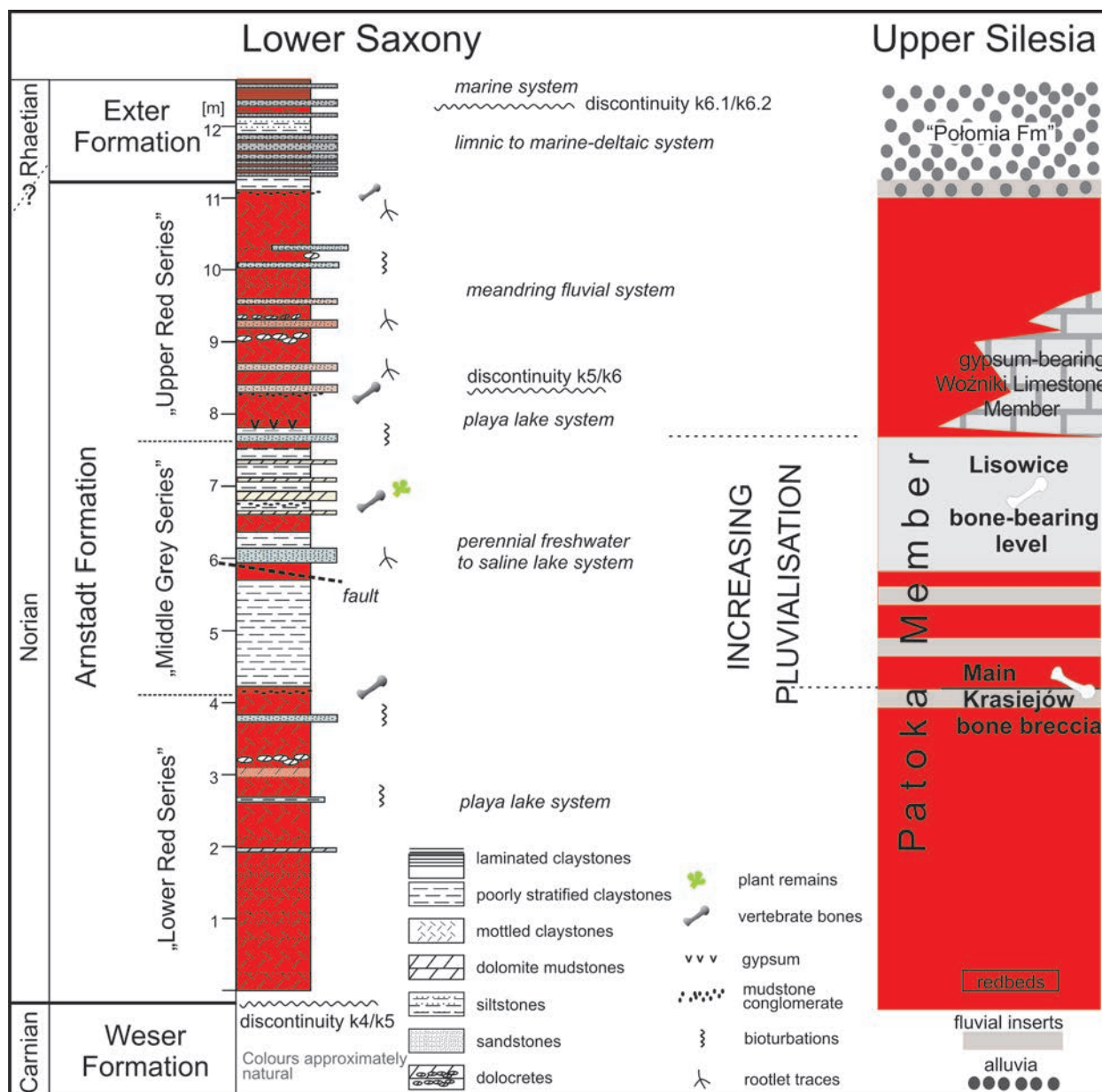
Fig. 20. Stratigraphic correlation of Upper Silesian vertebrate-bearing levels with an appropriate German middle Keuper reference succession in Lower Saxony (after Arp et al. , 2005, fig. 2). Note that only major Krasiejów bone-rich horizons are shown (see Fig. 3).
