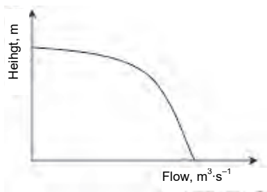
Fig. 3. The characteristic curve, describing the relationship between the discharge head and the flow, with the function H = f(Q) ; source: own elaboration
