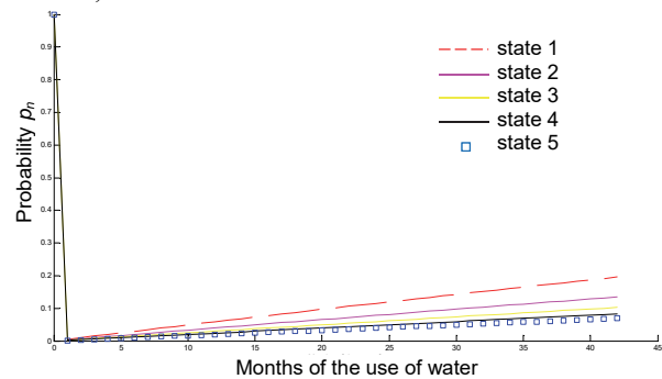
Fig. 6. Variation of the transition probability of the states, for the discharge head (the coefficient of storage is k = 84 ); p_n as in Fig. 4; source: own study
