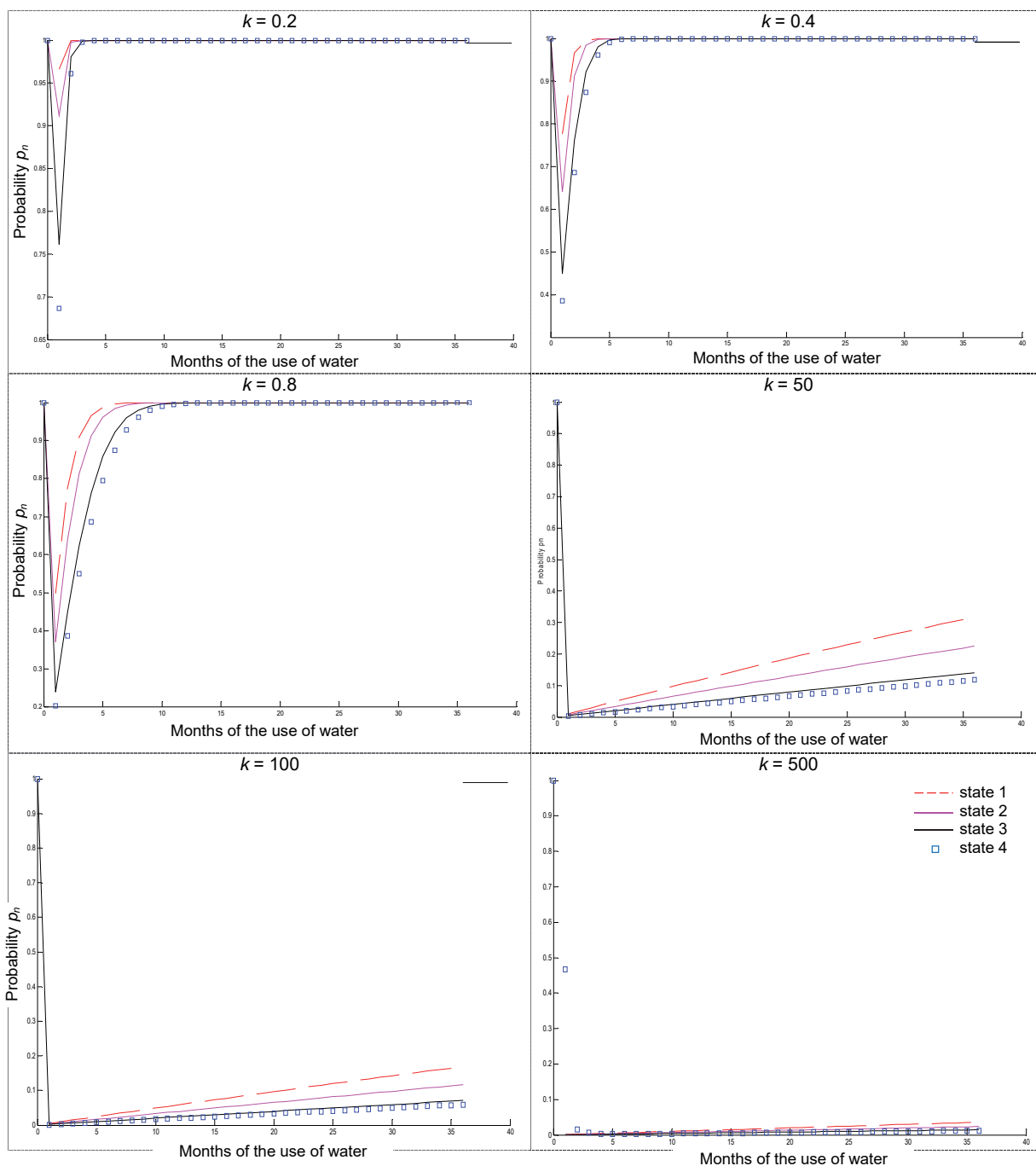
Fig. 5. Variation of the transition probability of the states, for the discharge head, for various coefficient of storage k ; p_n , as in Fig. 4; source: own study
