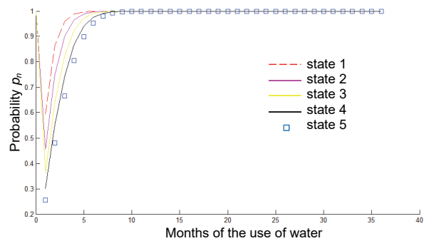
Fig. 4. Variation of the transition probability of the states, for the discharge head (the coefficient of storage is k = 0.62 ); p_n is calculated in the equation (16); source: own elaboration
