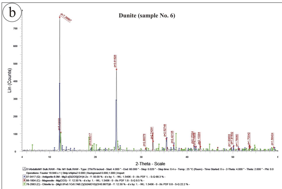
Text-fig. 3. a – Chart of X-ray diffraction analysis in the serpentinized harzburgite, and b – Chart of X-ray diffraction analysis in the serpentinized dunite
