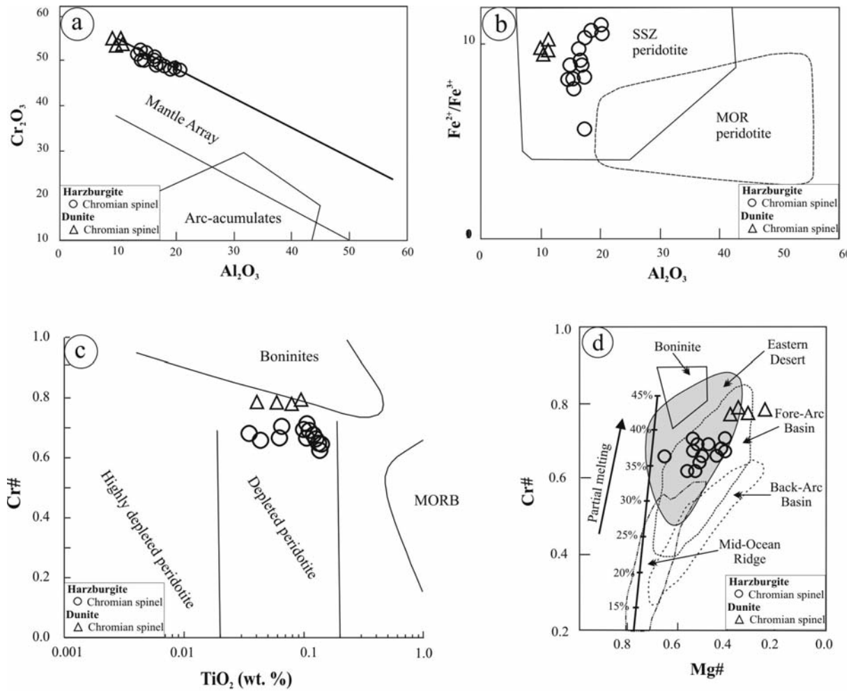
Text-fig. 6. (a -) Plot of fresh chromian spinels on Al_2O_3 vs. Cr_2O_3 diagram (after Franz and Wirth 2000), (b -) Al_2O_3 vs. Fe^{2+}/Fe^{3+} diagram showing the fields of supra-subduction zone (SSZ) and mid oceanic ridge (MOR) peridotite (after Kamenetsky et al. 2001), (c -) Cr# vs. TiO_2 diagram for the analyzed fresh chrome spinels (fields after Dick and Bullen 1984; Arai 1992; Jan and Windley 1990), and (d -) Cr# vs. Mg# diagram for fresh chromian spinels (after Stern et al. 2004); the field boundaries are from Dick and Bullen (1984), Bloomer et al. (1995) and Ohara et al. (2002). The melting trend of experimental equilibrium (melting %) is from Hirose and Kawamoto (1995). Field for chromites in the Egyptian serpentinites of the Eastern Desert is adopted from Farahat et al. (2011)
