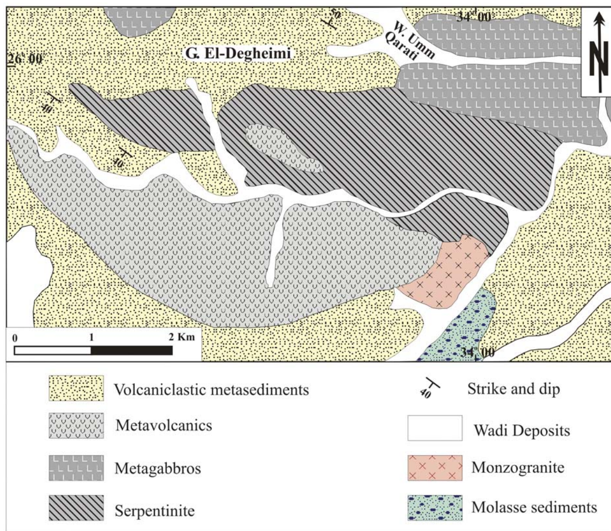
Text-fig. 2. Detailed geological map of the Gabal El-Degheimi area (after Akaad and Abu El Ela 2002)
