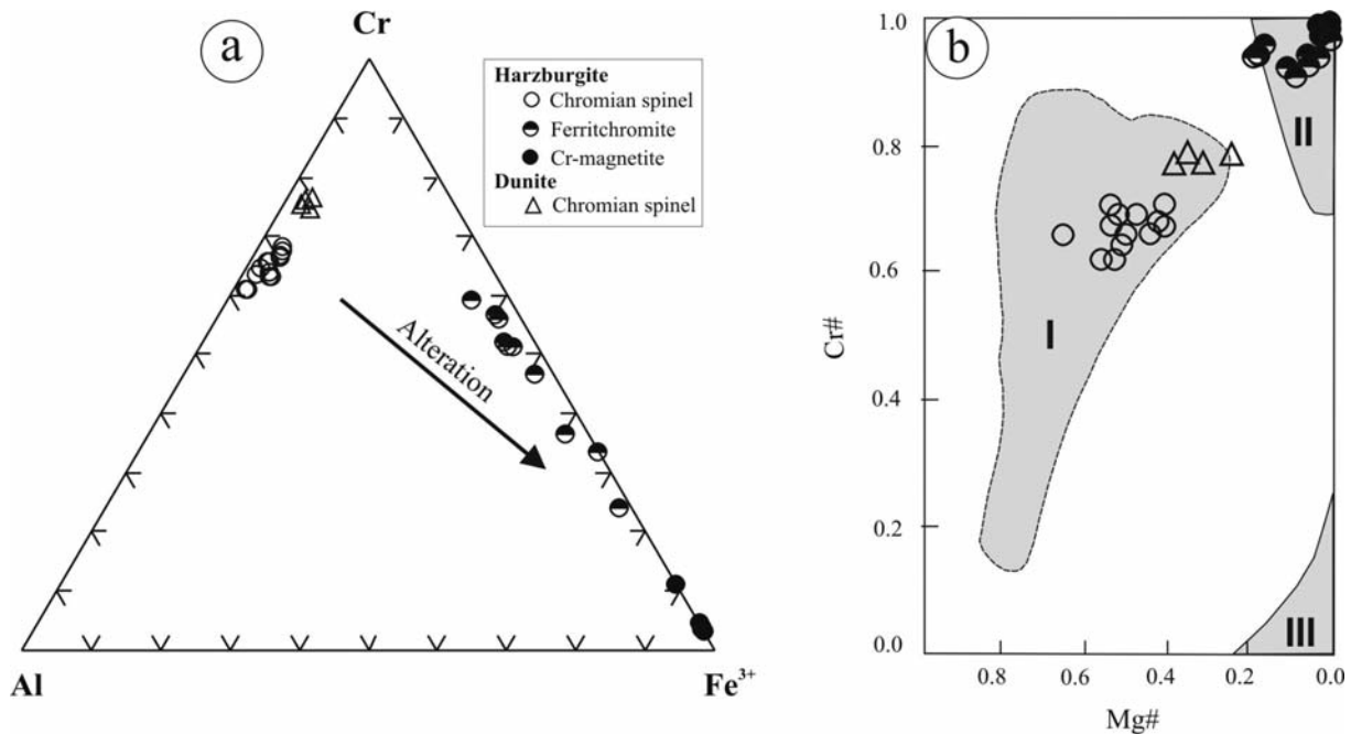
Text-fig. 5. a – Cr–Al–Fe 3+ plot of chromian spinels and their alteration products, and b – Mg# vs. Cr# variation diagram (fields after Roeder 1994 and Mondal et al. 2001). Field I: Cr-spinels in mantle peridotites, field II: magnetite from metamorphic rocks, field III: magnetite from unmetamorphosed igneous rocks
