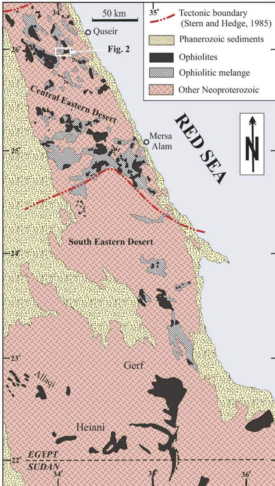
Text-fig. 1. Distribution of ophiolitic rocks in the Eastern Desert of Egypt (modified after Shackleton 1994). The location of Figure 2 is indicated
