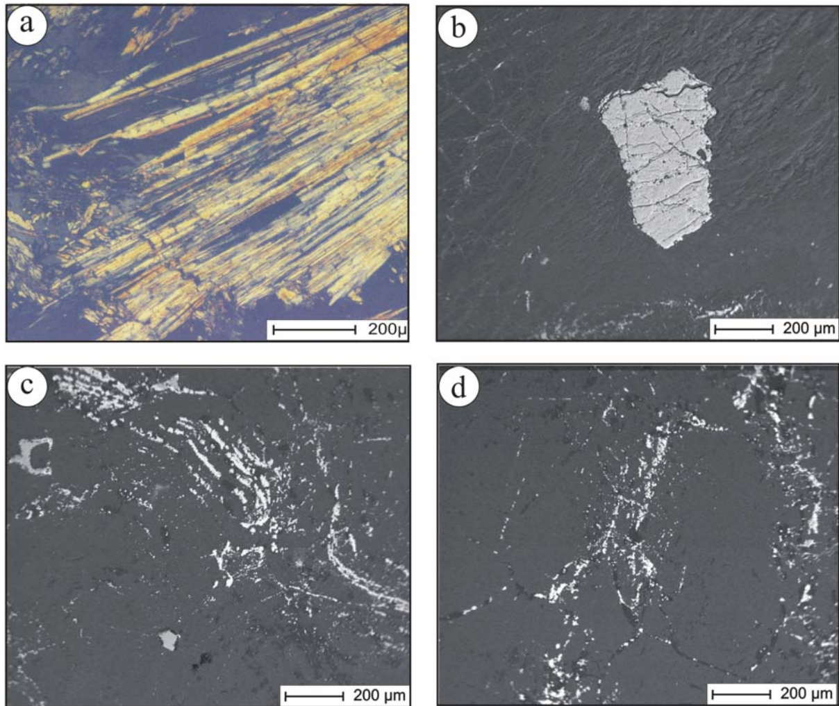
Text-fig. 4. a – long needles of anthophyllite near the contact with monzogranite (under crossed nichols), b – Backscattered-electron (BSE) image showing disseminated chromian spinel in the serpentinites, c – BSE image showing thin magnetite streaks and striations disposed along the cleavage planes of original orthopyroxene, and d – BSE image showing fine magnetite clusters surrounding olivine crystals
