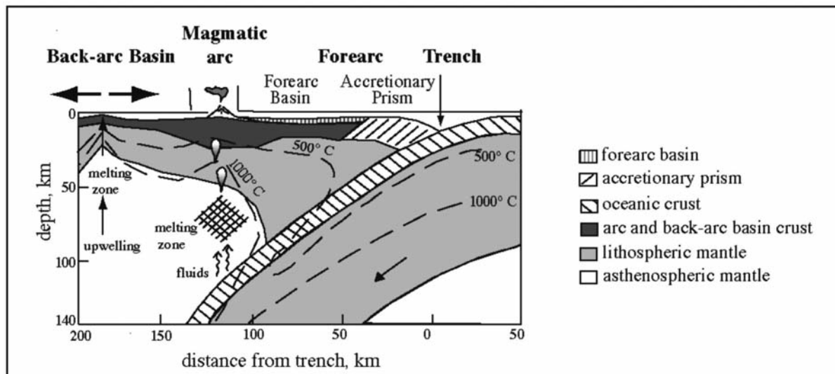
Text-fig. 7. Cartoons showing the tectonic setting of Egyptian ophiolites in the fore-arc environment above subduction zones (after Azer and Stern 2007)
