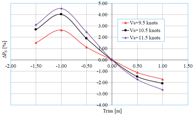
Fig. 7. The percentage changes of main engine power at different trims relative to even keel condition in case study 1
