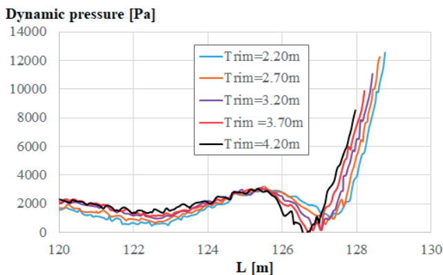
Fig. 13. Comparison of dynamic pressure distribution on fore-body in case study 2 at V=11.05 knots
