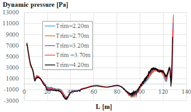
Fig. 11. Comparison of dynamic pressure distribution on hull surface at Z=2.7 m in case study 2 with V=11.05 knots
