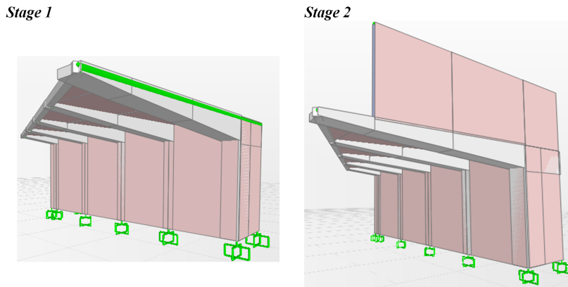
Figure 11. The staged construction of the cantilever parts
