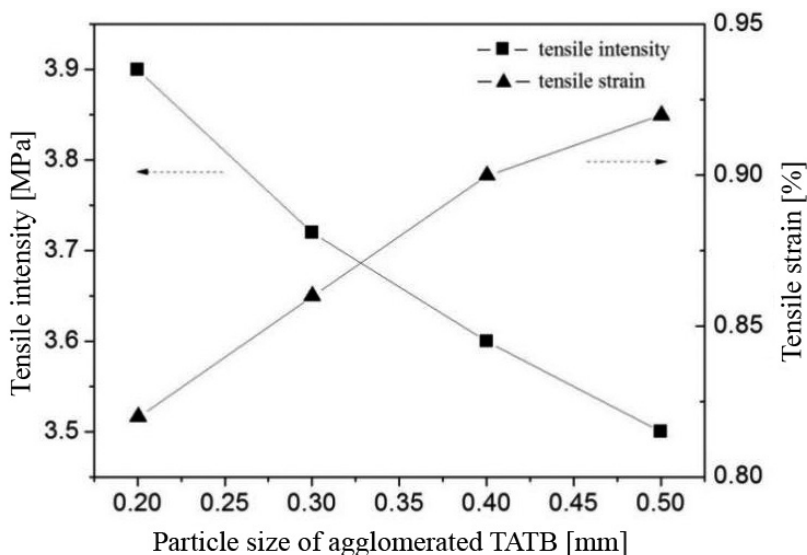
Figure 5. Tensile properties of PBX 2, PBX-5, PBX-6 and PBX-7 with different agglomerated TATB particle sizes
